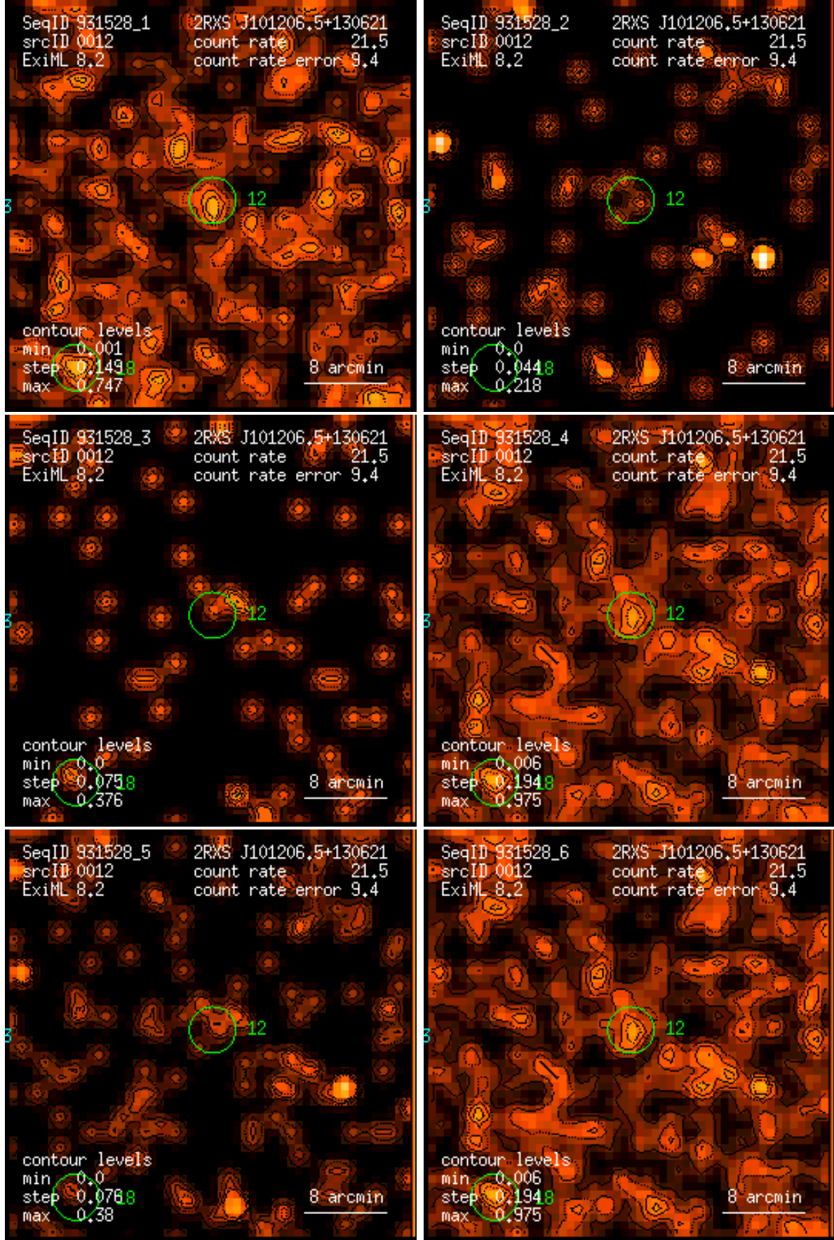
Figure 12: RASS 931528: detection 0012: band rate images, Gaussian filter: (1) PSPC channels 11 – 41, (2) 52 – 90, (3) 91 – 201, (4) 11 – 235, (5) 52 – 201, (6) 11 – 201. Broad band rates in counts/ks. Band rate contour levels in counts/ks/arcmin 2 .
