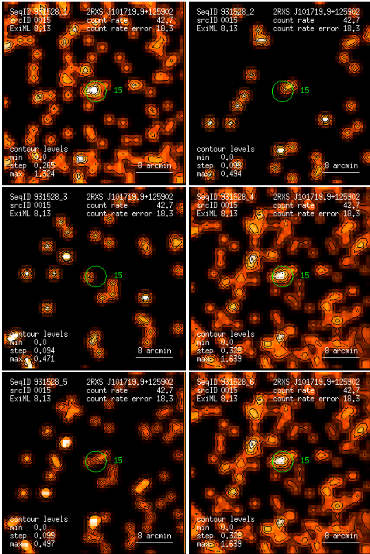
Figure 15: RASS 931528: detection 0015: band rate images, Gaussian filter: (1) PSPC channels 11 – 41, (2) 52 – 90, (3) 91 – 201, (4) 11 – 235, (5) 52 – 201, (6) 11 – 201. Broad band rates in counts/ks. Band rate contour levels in counts/ks/arcmin 2 .
