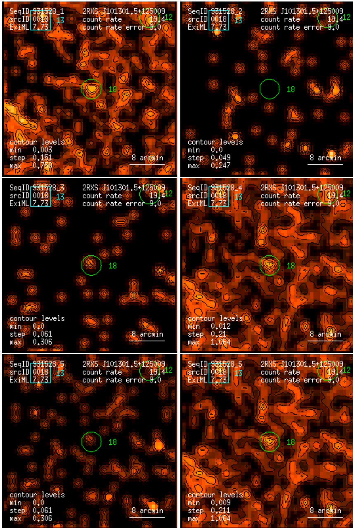
Figure 18: RASS 931528: detection 0018: band rate images, Gaussian filter: (1) PSPC channels 11 – 41, (2) 52 – 90, (3) 91 – 201, (4) 11 – 235, (5) 52 – 201, (6) 11 – 201. Broad band rates in counts/ks. Band rate contour levels in counts/ks/arcmin 2 .
