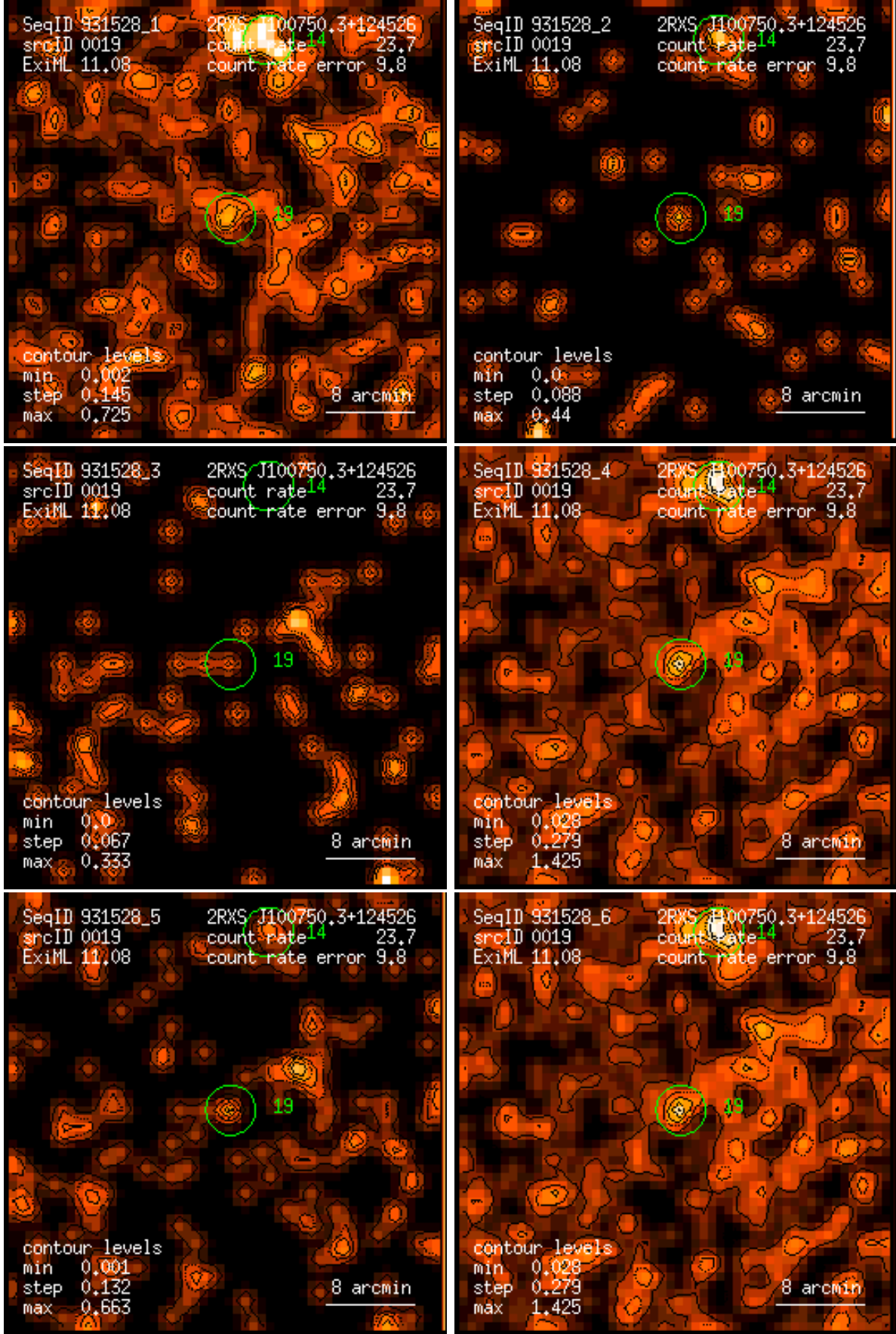
Figure 19: RASS 931528: detection 0019: band rate images, Gaussian filter: (1) PSPC channels 11 – 41, (2) 52 – 90, (3) 91 – 201, (4) 11 – 235, (5) 52 – 201, (6) 11 – 201. Broad band rates in counts/ks. Band rate contour levels in counts/ks/arcmin 2 .
