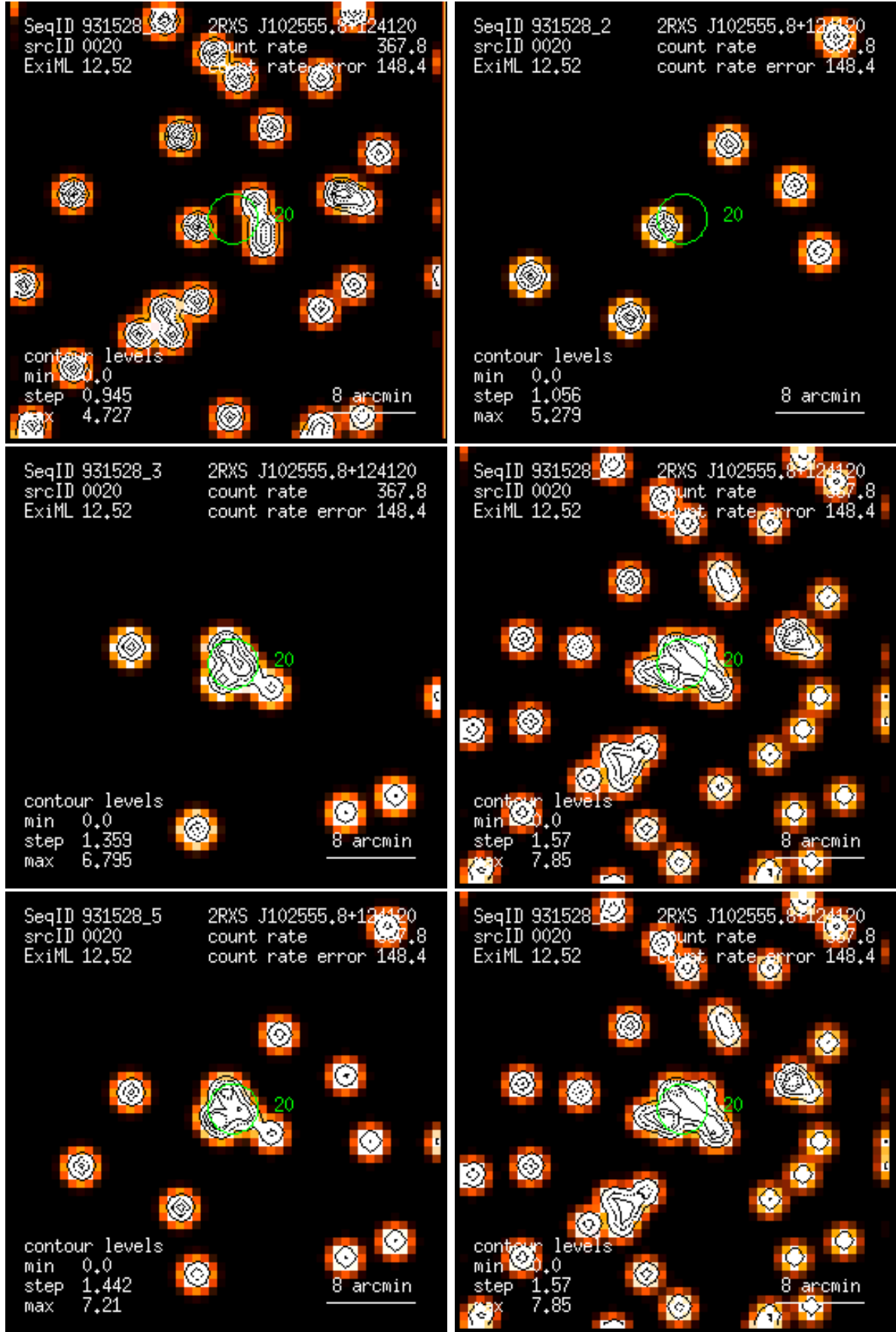
Figure 20: RASS 931528: detection 0020: band rate images, Gaussian filter: (1) PSPC channels 11 – 41, (2) 52 – 90, (3) 91 – 201, (4) 11 – 235, (5) 52 – 201, (6) 11 – 201. Broad band rates in counts/ks. Band rate contour levels in counts/ks/arcmin 2 .
