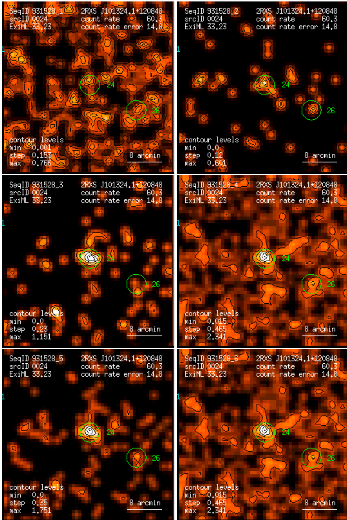
Figure 24: RASS 931528: detection 0024: band rate images, Gaussian filter: (1) PSPC channels 11 – 41, (2) 52 – 90, (3) 91 – 201, (4) 11 – 235, (5) 52 – 201, (6) 11 – 201. Broad band rates in counts/ks. Band rate contour levels in counts/ks/arcmin 2 .
