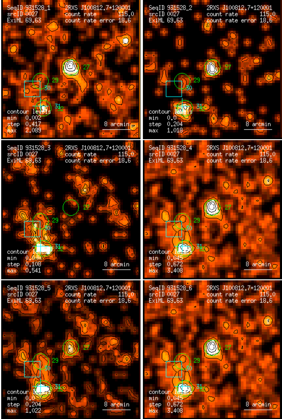
Figure 27: RASS 931528: detection 0027: band rate images, Gaussian filter: (1) PSPC channels 11 – 41, (2) 52 – 90, (3) 91 – 201, (4) 11 – 235, (5) 52 – 201, (6) 11 – 201. Broad band rates in counts/ks. Band rate contour levels in counts/ks/arcmin 2 .
