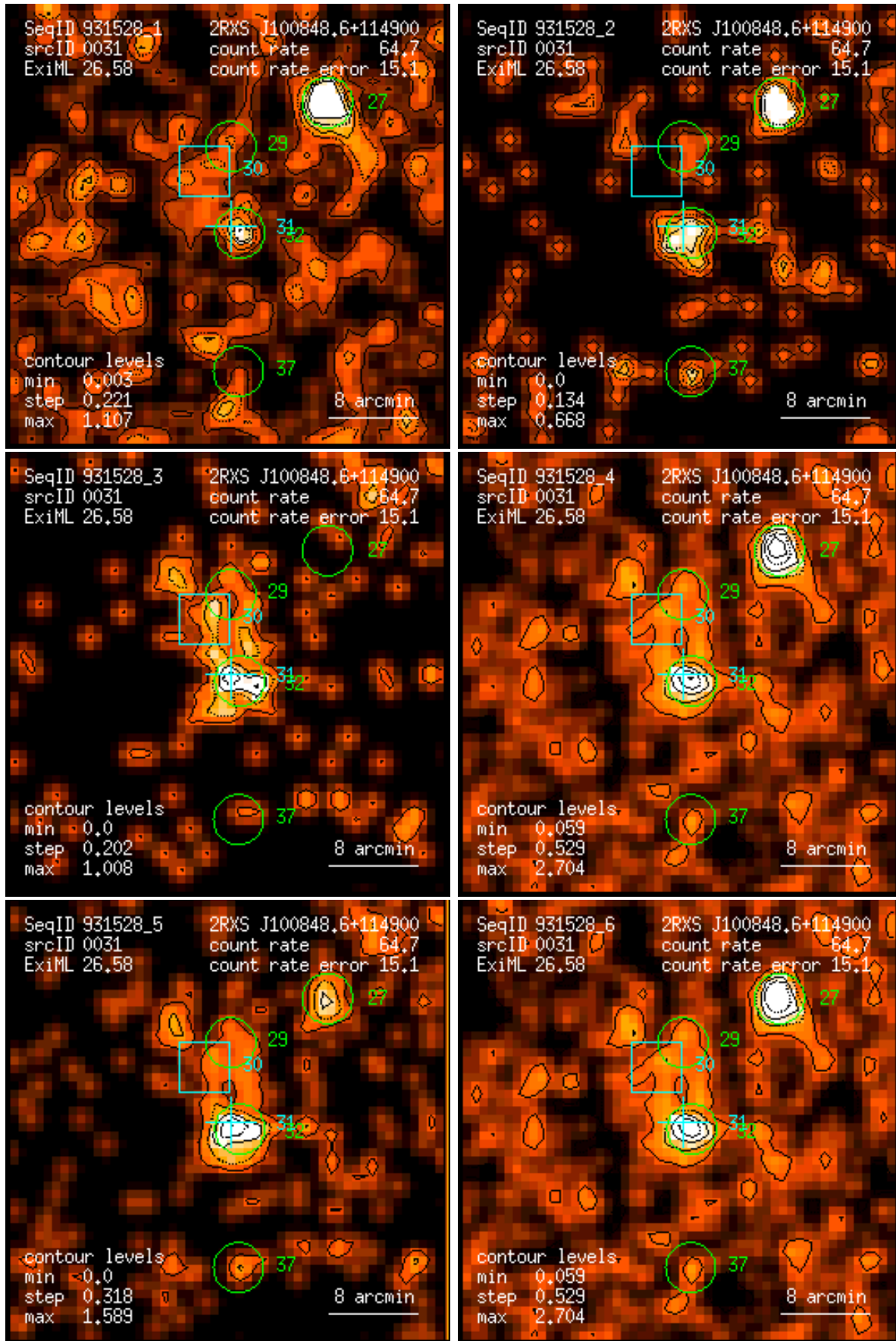
Figure 31: RASS 931528: detection 0031: band rate images, Gaussian filter: (1) PSPC channels 11 – 41, (2) 52 – 90, (3) 91 – 201, (4) 11 – 235, (5) 52 – 201, (6) 11 – 201. Broad band rates in counts/ks. Band rate contour levels in counts/ks/arcmin 2 .
