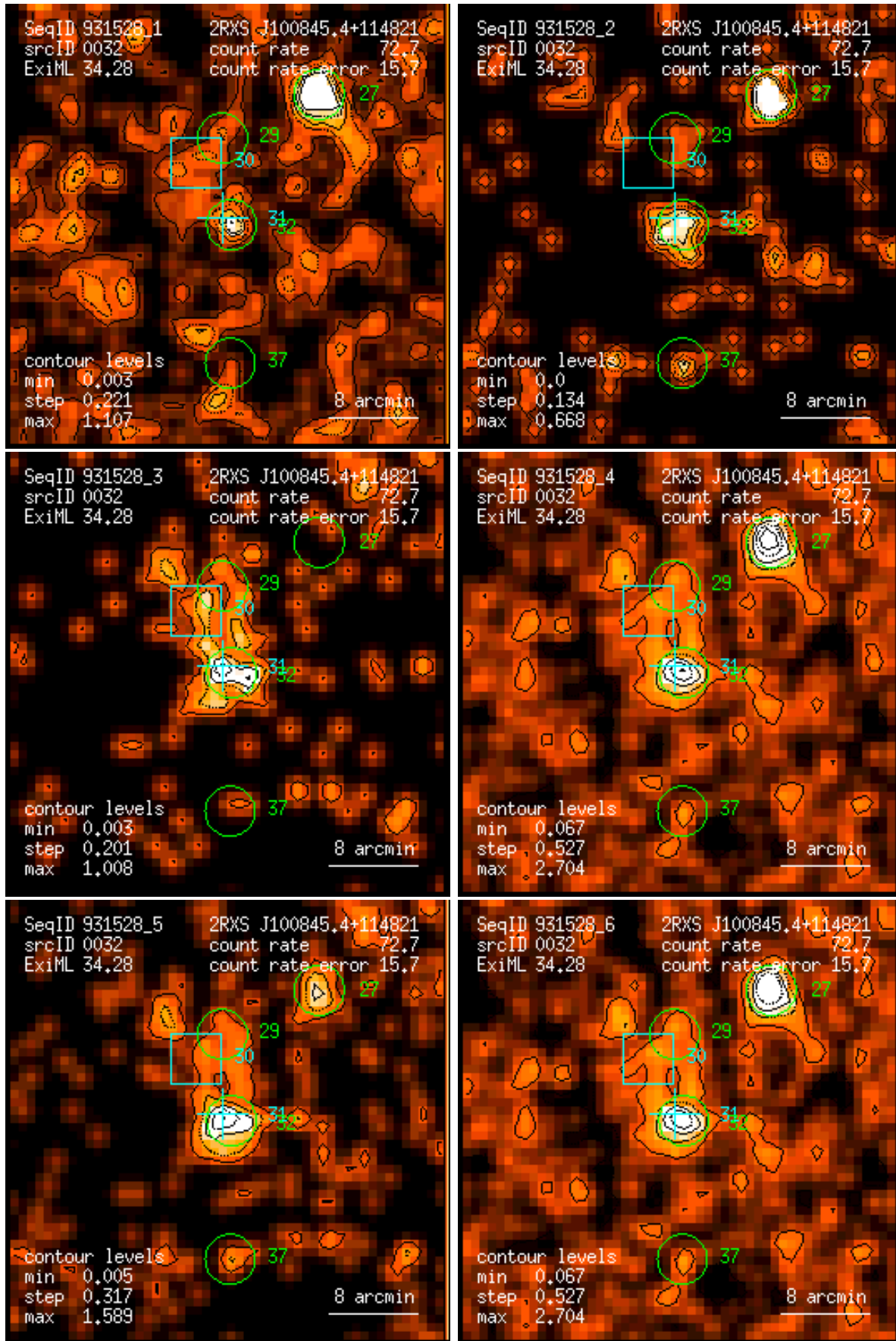
Figure 32: RASS 931528: detection 0032: band rate images, Gaussian filter: (1) PSPC channels 11 – 41, (2) 52 – 90, (3) 91 – 201, (4) 11 – 235, (5) 52 – 201, (6) 11 – 201. Broad band rates in counts/ks. Band rate contour levels in counts/ks/arcmin 2 .
