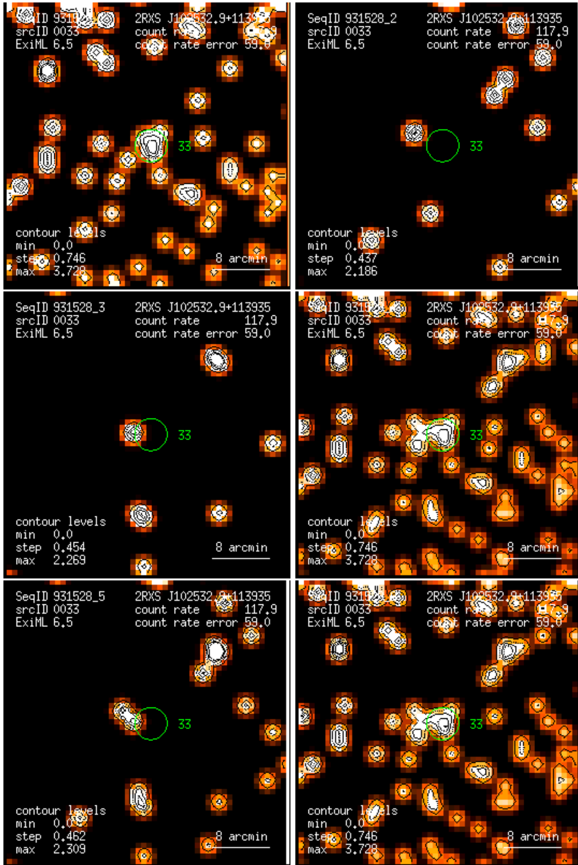
Figure 33: RASS 931528: detection 0033: band rate images, Gaussian filter: (1) PSPC channels 11 – 41, (2) 52 – 90, (3) 91 – 201, (4) 11 – 235, (5) 52 – 201, (6) 11 – 201. Broad band rates in counts/ks. Band rate contour levels in counts/ks/arcmin 2 .
