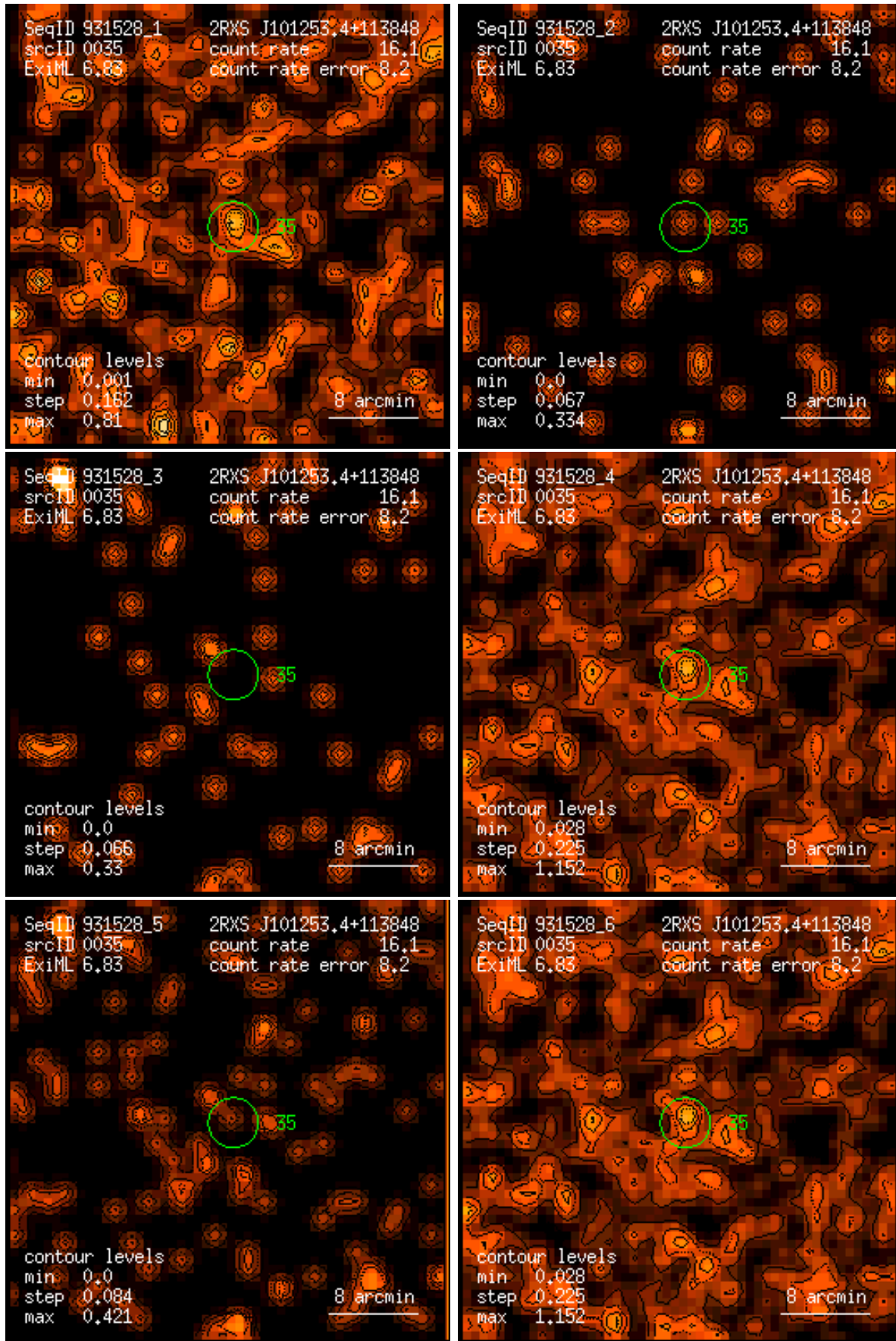
Figure 35: RASS 931528: detection 0035: band rate images, Gaussian filter: (1) PSPC channels 11 – 41, (2) 52 – 90, (3) 91 – 201, (4) 11 – 235, (5) 52 – 201, (6) 11 – 201. Broad band rates in counts/ks. Band rate contour levels in counts/ks/arcmin 2 .
