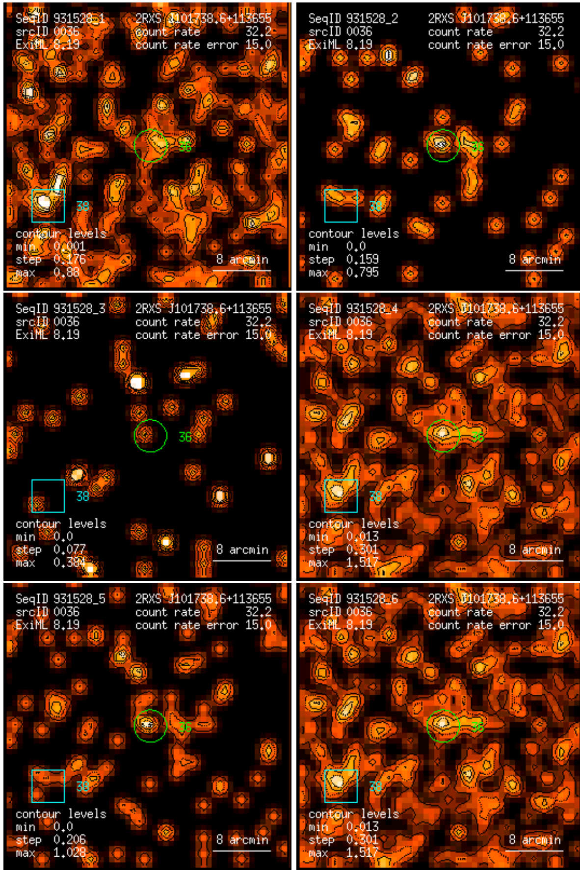
Figure 36: RASS 931528: detection 0036: band rate images, Gaussian filter: (1) PSPC channels 11 – 41, (2) 52 – 90, (3) 91 – 201, (4) 11 – 235, (5) 52 – 201, (6) 11 – 201. Broad band rates in counts/ks. Band rate contour levels in counts/ks/arcmin 2 .
