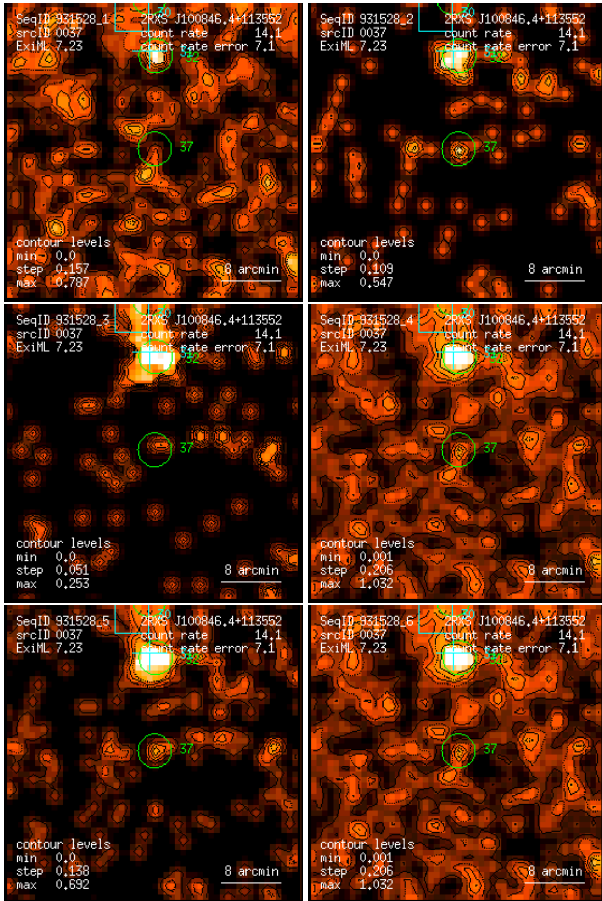
Figure 37: RASS 931528: detection 0037: band rate images, Gaussian filter: (1) PSPC channels 11 – 41, (2) 52 – 90, (3) 91 – 201, (4) 11 – 235, (5) 52 – 201, (6) 11 – 201. Broad band rates in counts/ks. Band rate contour levels in counts/ks/arcmin 2 .
