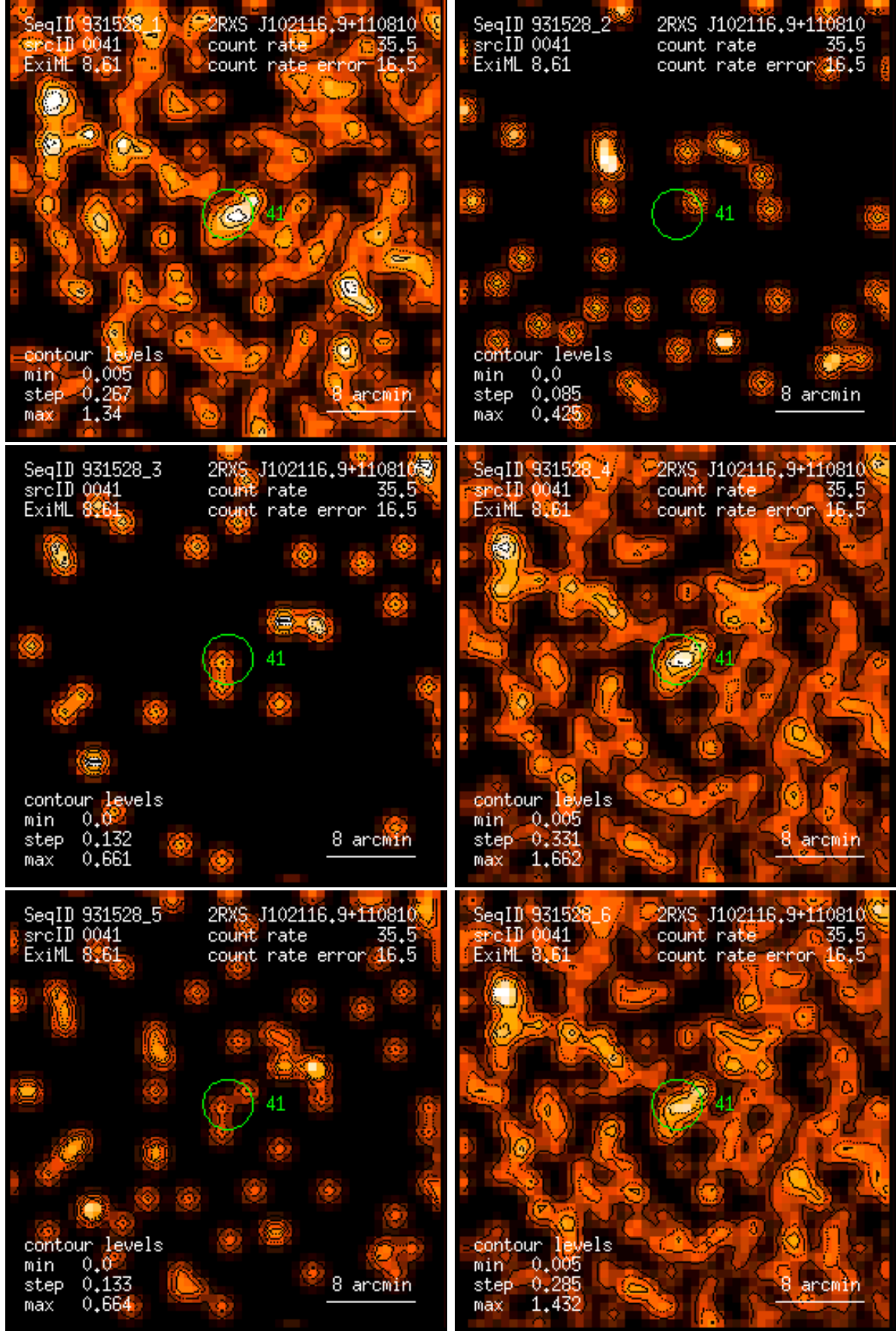
Figure 41: RASS 931528: detection 0041: band rate images, Gaussian filter: (1) PSPC channels 11 – 41, (2) 52 – 90, (3) 91 – 201, (4) 11 – 235, (5) 52 – 201, (6) 11 – 201. Broad band rates in counts/ks. Band rate contour levels in counts/ks/arcmin 2 .
