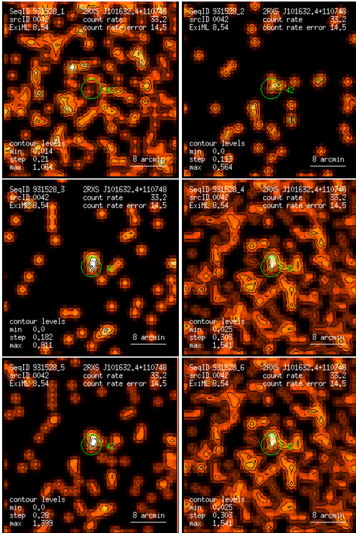
Figure 42: RASS 931528: detection 0042: band rate images, Gaussian filter: (1) PSPC channels 11 – 41, (2) 52 – 90, (3) 91 – 201, (4) 11 – 235, (5) 52 – 201, (6) 11 – 201. Broad band rates in counts/ks. Band rate contour levels in counts/ks/arcmin 2 .
