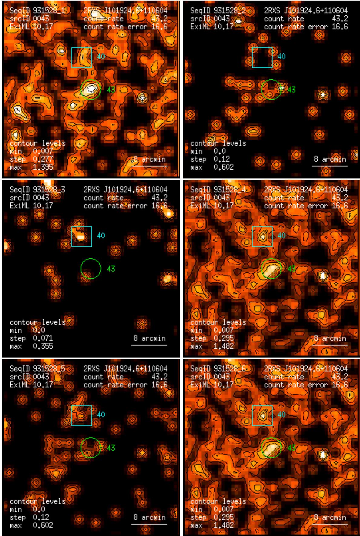
Figure 43: RASS 931528: detection 0043: band rate images, Gaussian filter: (1) PSPC channels 11 – 41, (2) 52 – 90, (3) 91 – 201, (4) 11 – 235, (5) 52 – 201, (6) 11 – 201. Broad band rates in counts/ks. Band rate contour levels in counts/ks/arcmin 2 .
