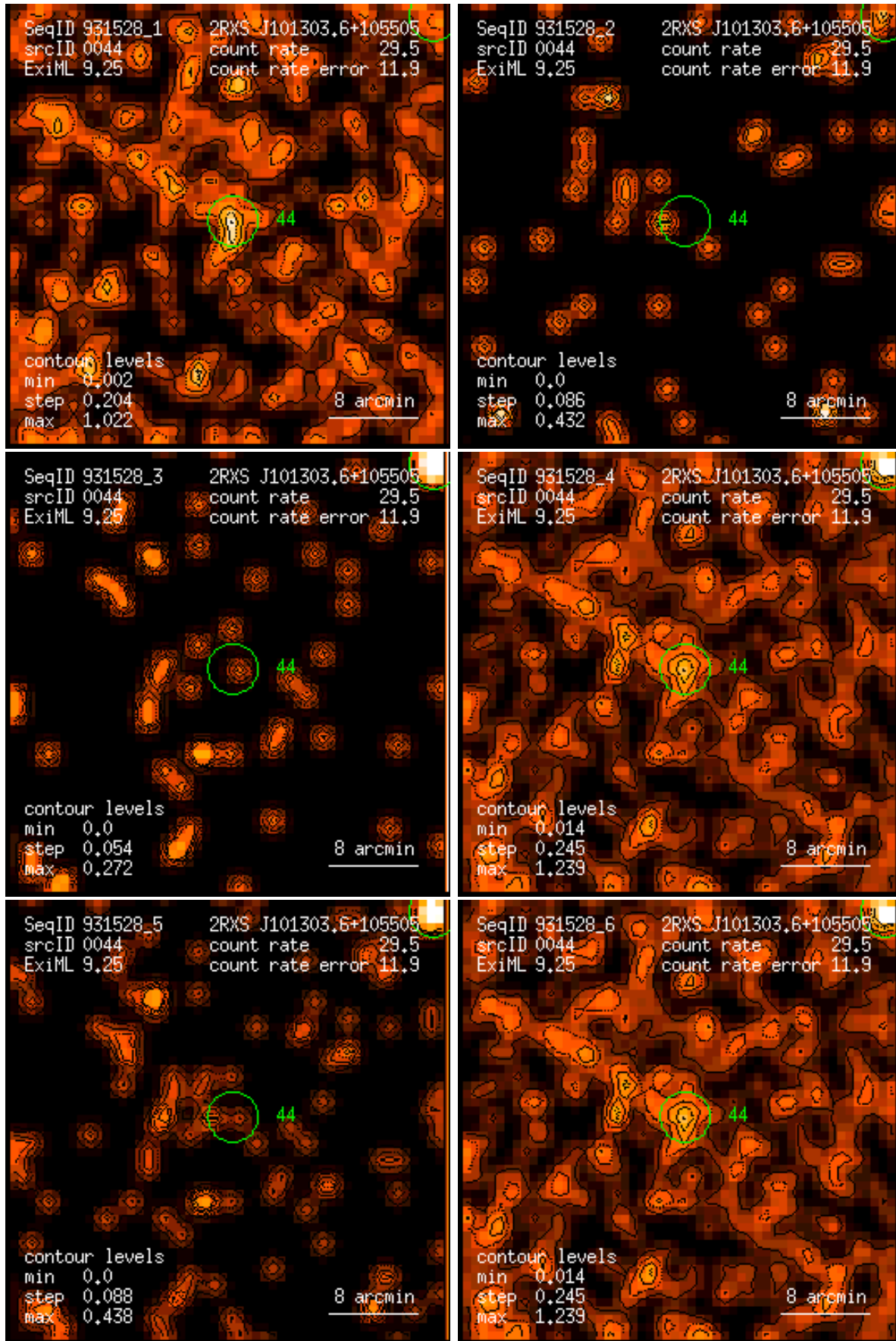
Figure 44: RASS 931528: detection 0044: band rate images, Gaussian filter: (1) PSPC channels 11 – 41, (2) 52 – 90, (3) 91 – 201, (4) 11 – 235, (5) 52 – 201, (6) 11 – 201. Broad band rates in counts/ks. Band rate contour levels in counts/ks/arcmin 2 .
