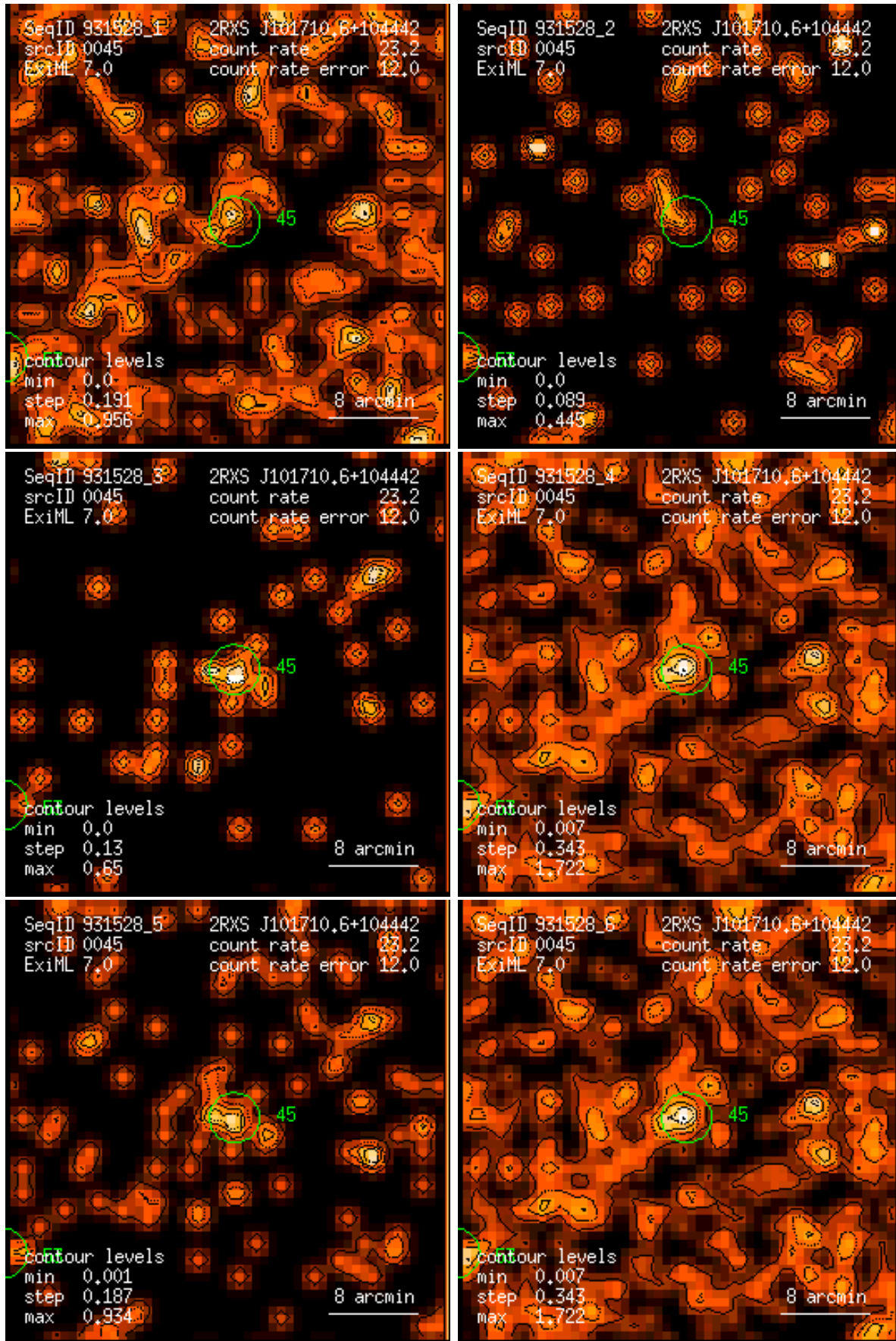
Figure 45: RASS 931528: detection 0045: band rate images, Gaussian filter: (1) PSPC channels 11 – 41, (2) 52 – 90, (3) 91 – 201, (4) 11 – 235, (5) 52 – 201, (6) 11 – 201. Broad band rates in counts/ks. Band rate contour levels in counts/ks/arcmin 2 .
