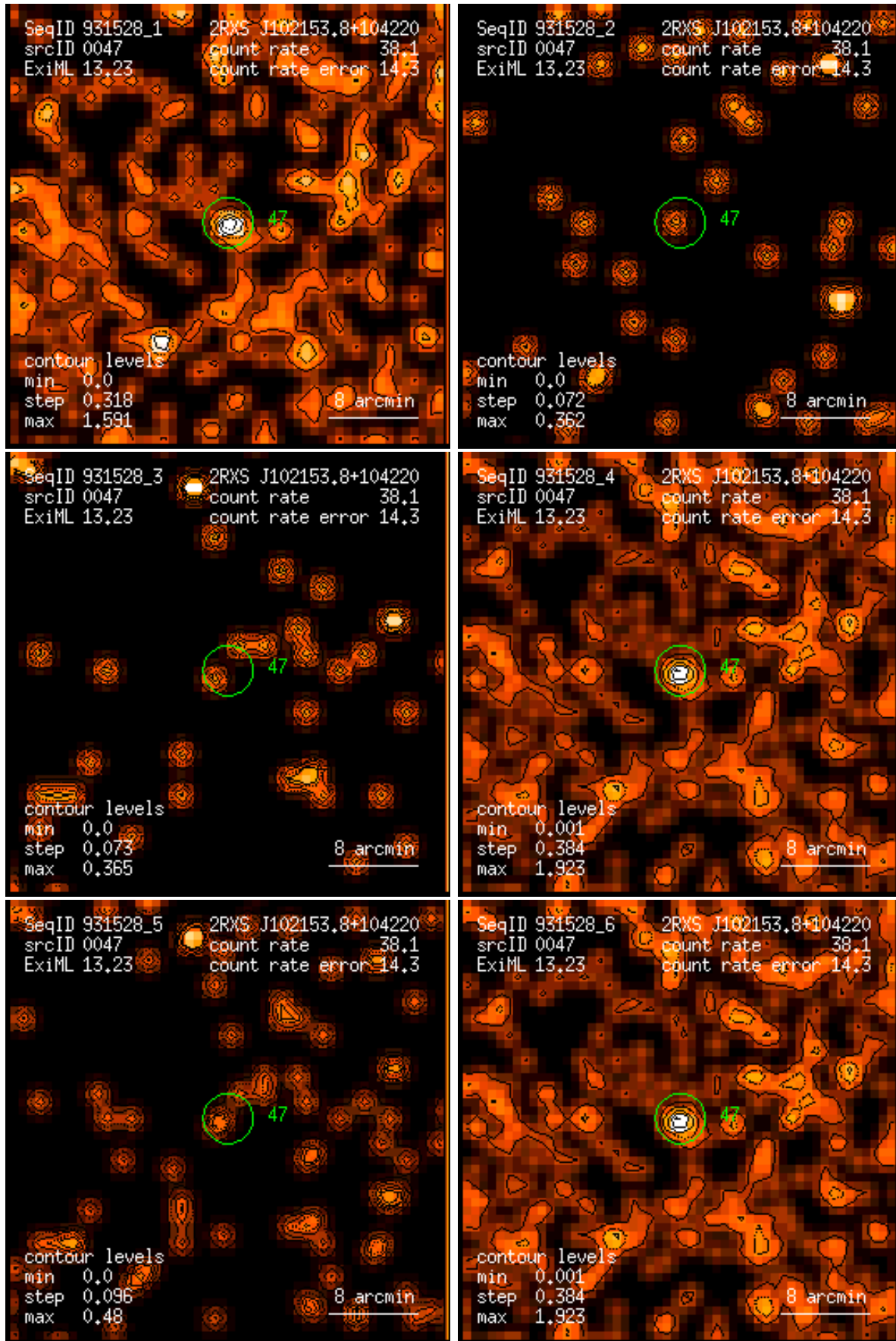
Figure 47: RASS 931528: detection 0047: band rate images, Gaussian filter: (1) PSPC channels 11 – 41, (2) 52 – 90, (3) 91 – 201, (4) 11 – 235, (5) 52 – 201, (6) 11 – 201. Broad band rates in counts/ks. Band rate contour levels in counts/ks/arcmin 2 .
