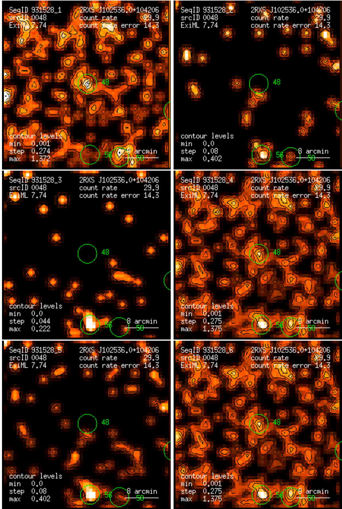
Figure 48: RASS 931528: detection 0048: band rate images, Gaussian filter: (1) PSPC channels 11 – 41, (2) 52 – 90, (3) 91 – 201, (4) 11 – 235, (5) 52 – 201, (6) 11 – 201. Broad band rates in counts/ks. Band rate contour levels in counts/ks/arcmin 2 .
