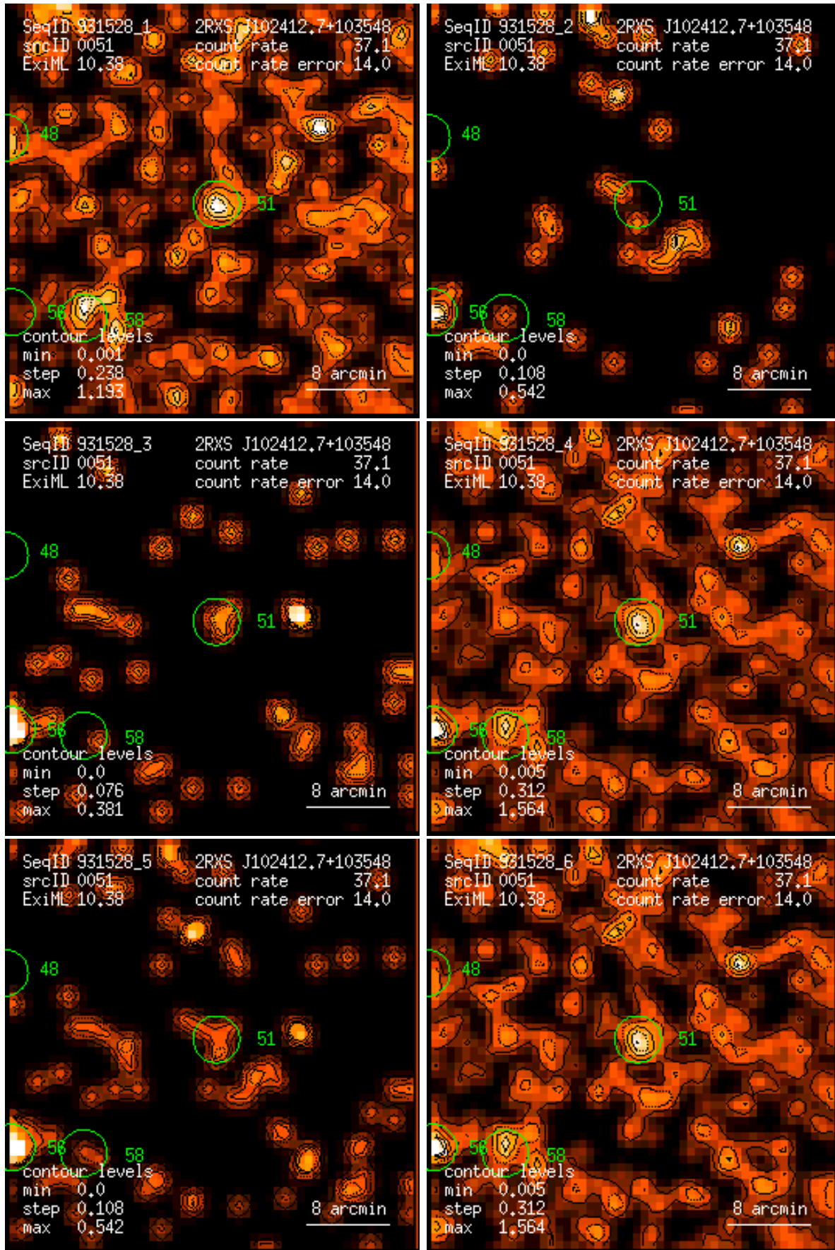
Figure 51: RASS 931528: detection 0051: band rate images, Gaussian filter: (1) PSPC channels 11 – 41, (2) 52 – 90, (3) 91 – 201, (4) 11 – 235, (5) 52 – 201, (6) 11 – 201. Broad band rates in counts/ks. Band rate contour levels in counts/ks/arcmin 2 .
