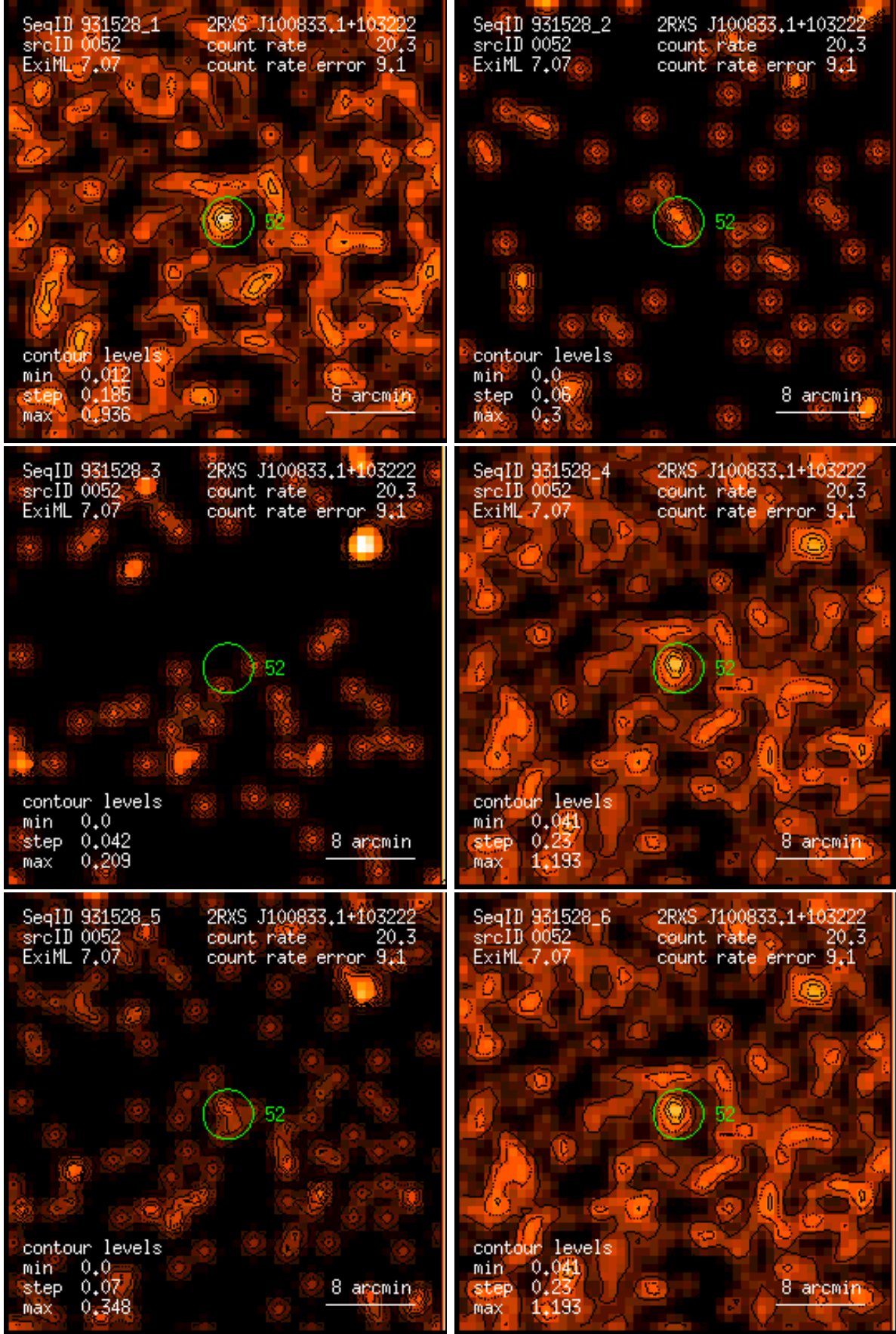
Figure 52: RASS 931528: detection 0052: band rate images, Gaussian filter: (1) PSPC channels 11 – 41, (2) 52 – 90, (3) 91 – 201, (4) 11 – 235, (5) 52 – 201, (6) 11 – 201. Broad band rates in counts/ks. Band rate contour levels in counts/ks/arcmin 2 .
