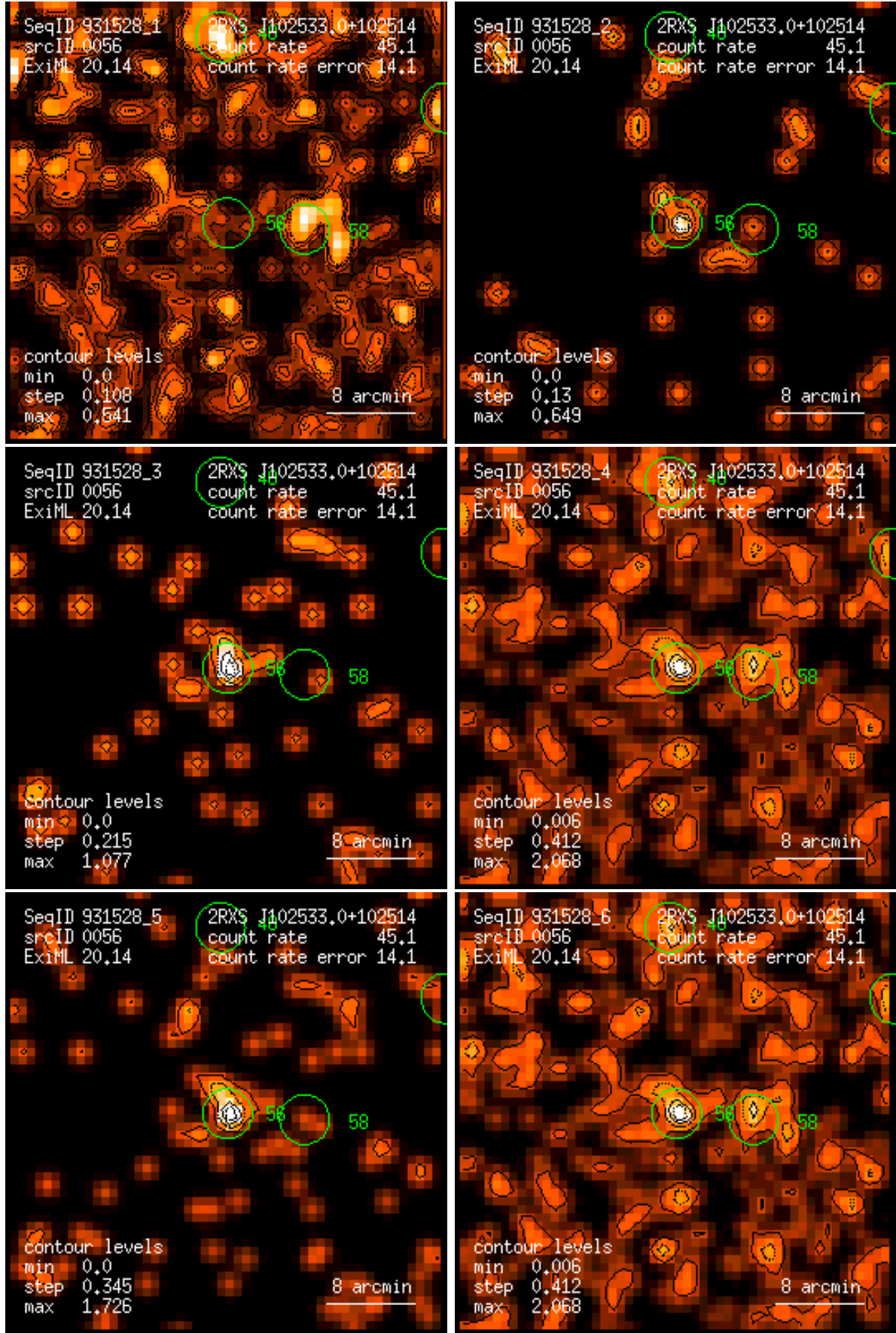
Figure 56: RASS 931528: detection 0056: band rate images, Gaussian filter: (1) PSPC channels 11 – 41, (2) 52 – 90, (3) 91 – 201, (4) 11 – 235, (5) 52 – 201, (6) 11 – 201. Broad band rates in counts/ks. Band rate contour levels in counts/ks/arcmin 2 .
