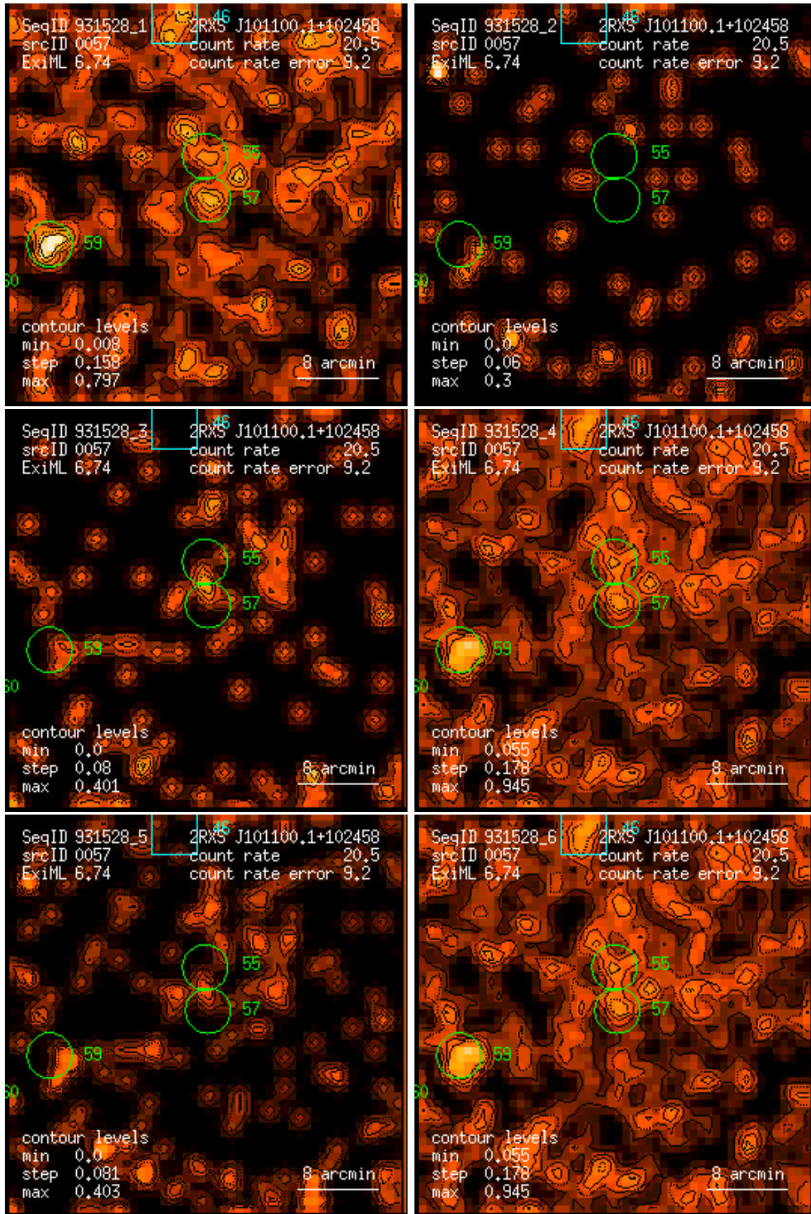
Figure 57: RASS 931528: detection 0057: band rate images, Gaussian filter: (1) PSPC channels 11 – 41, (2) 52 – 90, (3) 91 – 201, (4) 11 – 235, (5) 52 – 201, (6) 11 – 201. Broad band rates in counts/ks. Band rate contour levels in counts/ks/arcmin 2 .
