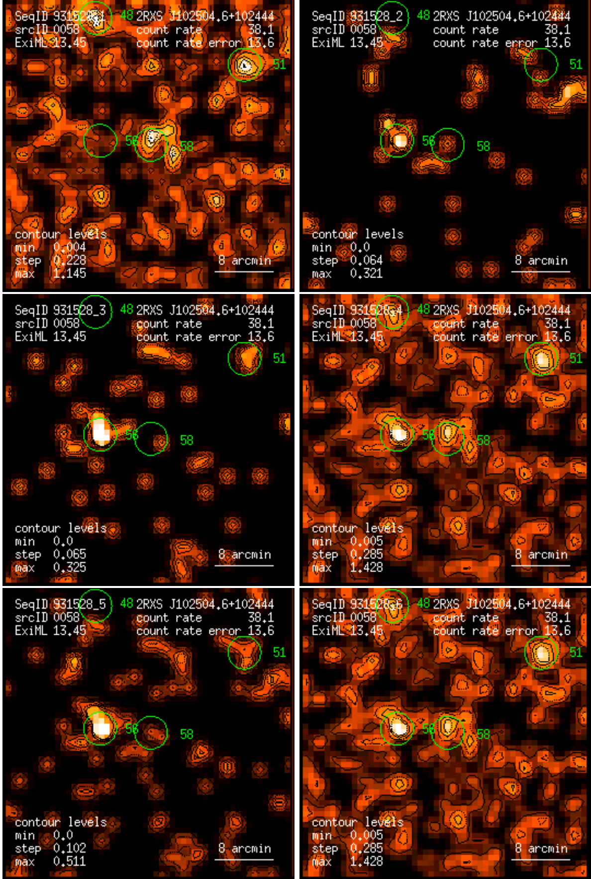
Figure 58: RASS 931528: detection 0058: band rate images, Gaussian filter: (1) PSPC channels 11 – 41, (2) 52 – 90, (3) 91 – 201, (4) 11 – 235, (5) 52 – 201, (6) 11 – 201. Broad band rates in counts/ks. Band rate contour levels in counts/ks/arcmin 2 .
