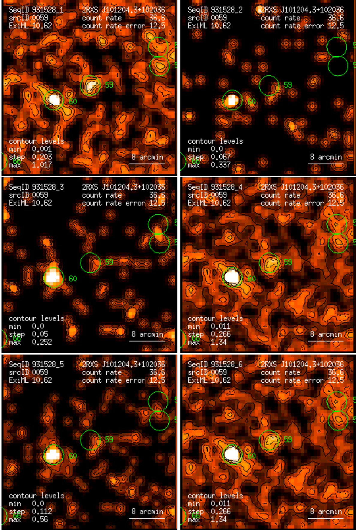
Figure 59: RASS 931528: detection 0059: band rate images, Gaussian filter: (1) PSPC channels 11 – 41, (2) 52 – 90, (3) 91 – 201, (4) 11 – 235, (5) 52 – 201, (6) 11 – 201. Broad band rates in counts/ks. Band rate contour levels in counts/ks/arcmin 2 .
