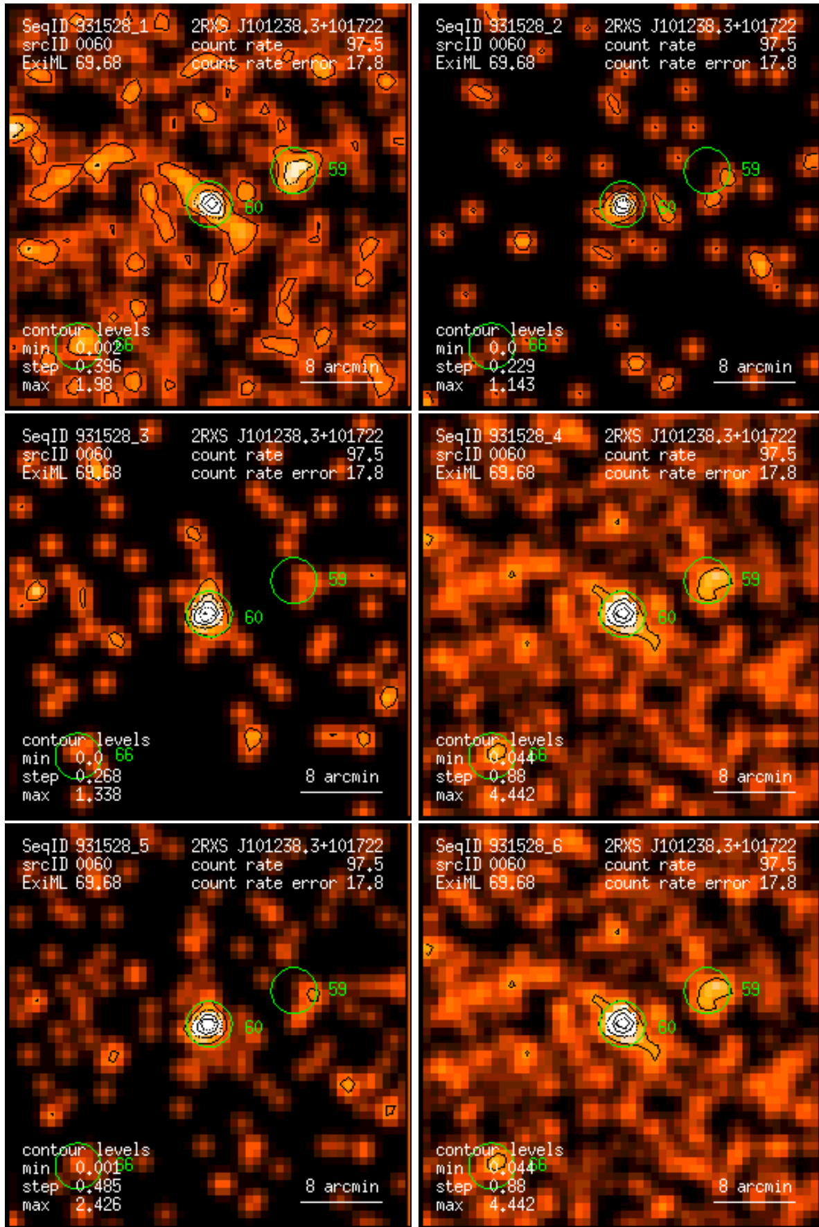
Figure 60: RASS 931528: detection 0060: band rate images, Gaussian filter: (1) PSPC channels 11 – 41, (2) 52 – 90, (3) 91 – 201, (4) 11 – 235, (5) 52 – 201, (6) 11 – 201. Broad band rates in counts/ks. Band rate contour levels in counts/ks/arcmin 2 .
