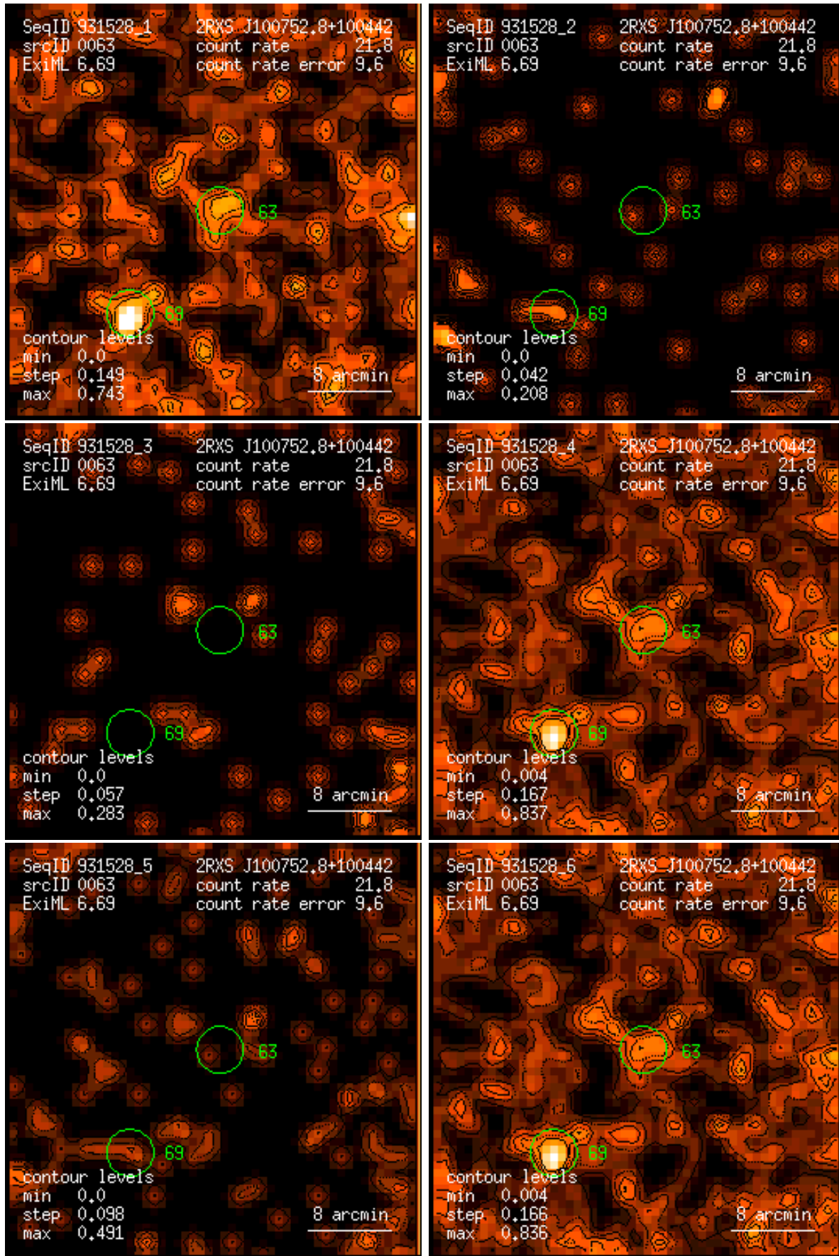
Figure 63: RASS 931528: detection 0063: band rate images, Gaussian filter: (1) PSPC channels 11 – 41, (2) 52 – 90, (3) 91 – 201, (4) 11 – 235, (5) 52 – 201, (6) 11 – 201. Broad band rates in counts/ks. Band rate contour levels in counts/ks/arcmin 2 .
