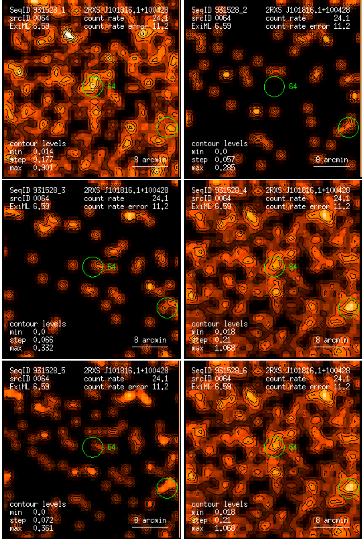
Figure 64: RASS 931528: detection 0064: band rate images, Gaussian filter: (1) PSPC channels 11 – 41, (2) 52 – 90, (3) 91 – 201, (4) 11 – 235, (5) 52 – 201, (6) 11 – 201. Broad band rates in counts/ks. Band rate contour levels in counts/ks/arcmin 2 .
