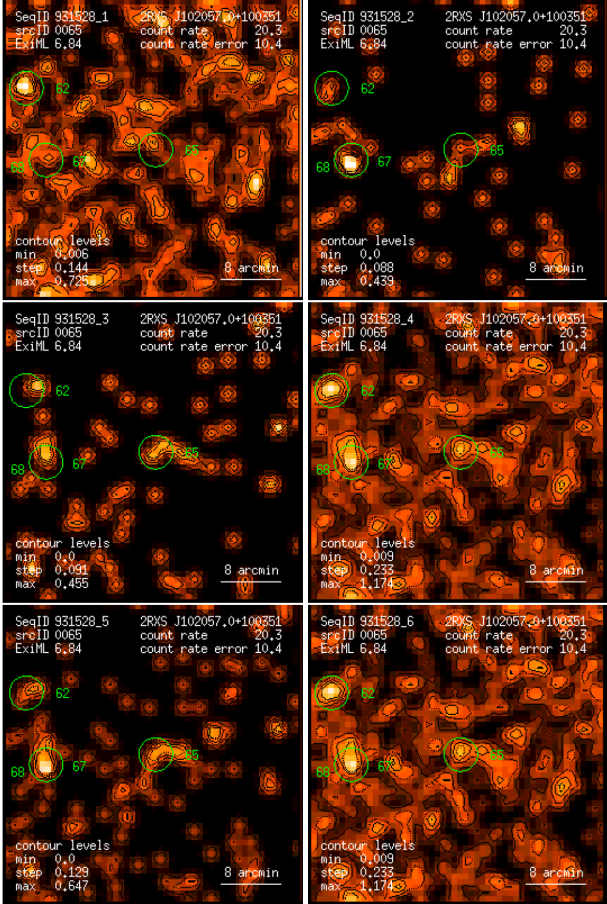
Figure 65: RASS 931528: detection 0065: band rate images, Gaussian filter: (1) PSPC channels 11 – 41, (2) 52 – 90, (3) 91 – 201, (4) 11 – 235, (5) 52 – 201, (6) 11 – 201. Broad band rates in counts/ks. Band rate contour levels in counts/ks/arcmin 2 .
