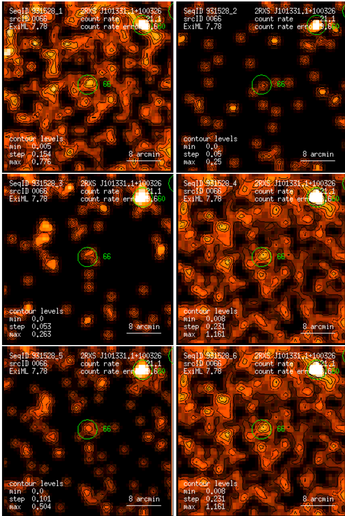
Figure 66: RASS 931528: detection 0066: band rate images, Gaussian filter: (1) PSPC channels 11 – 41, (2) 52 – 90, (3) 91 – 201, (4) 11 – 235, (5) 52 – 201, (6) 11 – 201. Broad band rates in counts/ks. Band rate contour levels in counts/ks/arcmin 2 .
