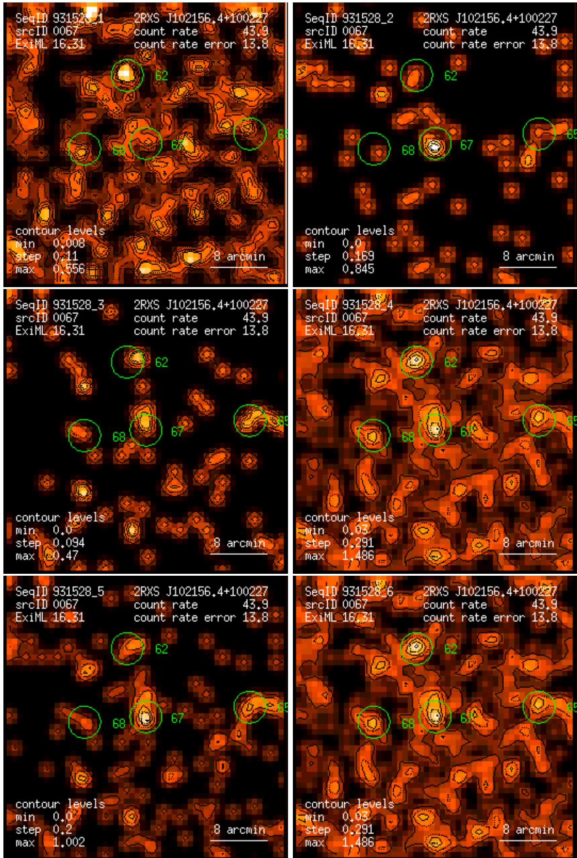
Figure 67: RASS 931528: detection 0067: band rate images, Gaussian filter: (1) PSPC channels 11 – 41, (2) 52 – 90, (3) 91 – 201, (4) 11 – 235, (5) 52 – 201, (6) 11 – 201. Broad band rates in counts/ks. Band rate contour levels in counts/ks/arcmin 2 .
