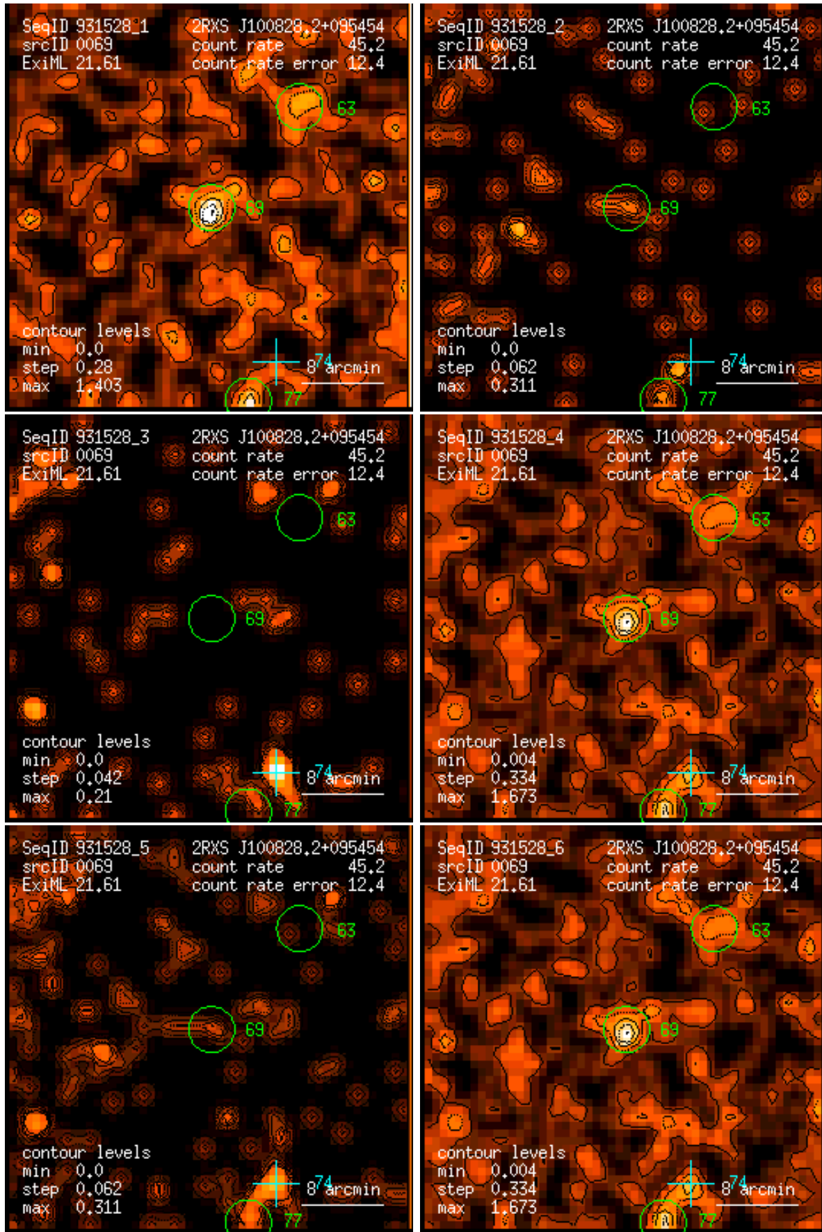
Figure 69: RASS 931528: detection 0069: band rate images, Gaussian filter: (1) PSPC channels 11 – 41, (2) 52 – 90, (3) 91 – 201, (4) 11 – 235, (5) 52 – 201, (6) 11 – 201. Broad band rates in counts/ks. Band rate contour levels in counts/ks/arcmin 2 .
