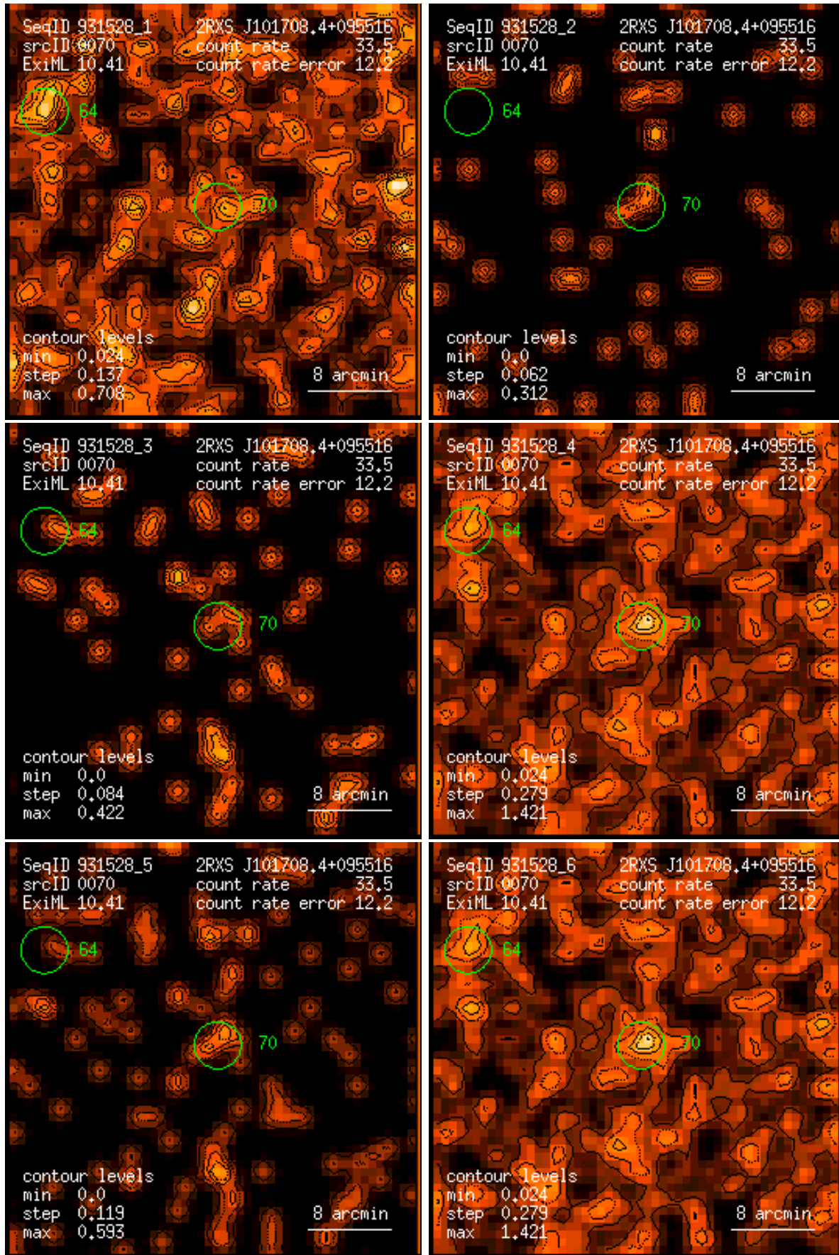
Figure 70: RASS 931528: detection 0070: band rate images, Gaussian filter: (1) PSPC channels 11 – 41, (2) 52 – 90, (3) 91 – 201, (4) 11 – 235, (5) 52 – 201, (6) 11 – 201. Broad band rates in counts/ks. Band rate contour levels in counts/ks/arcmin 2 .
