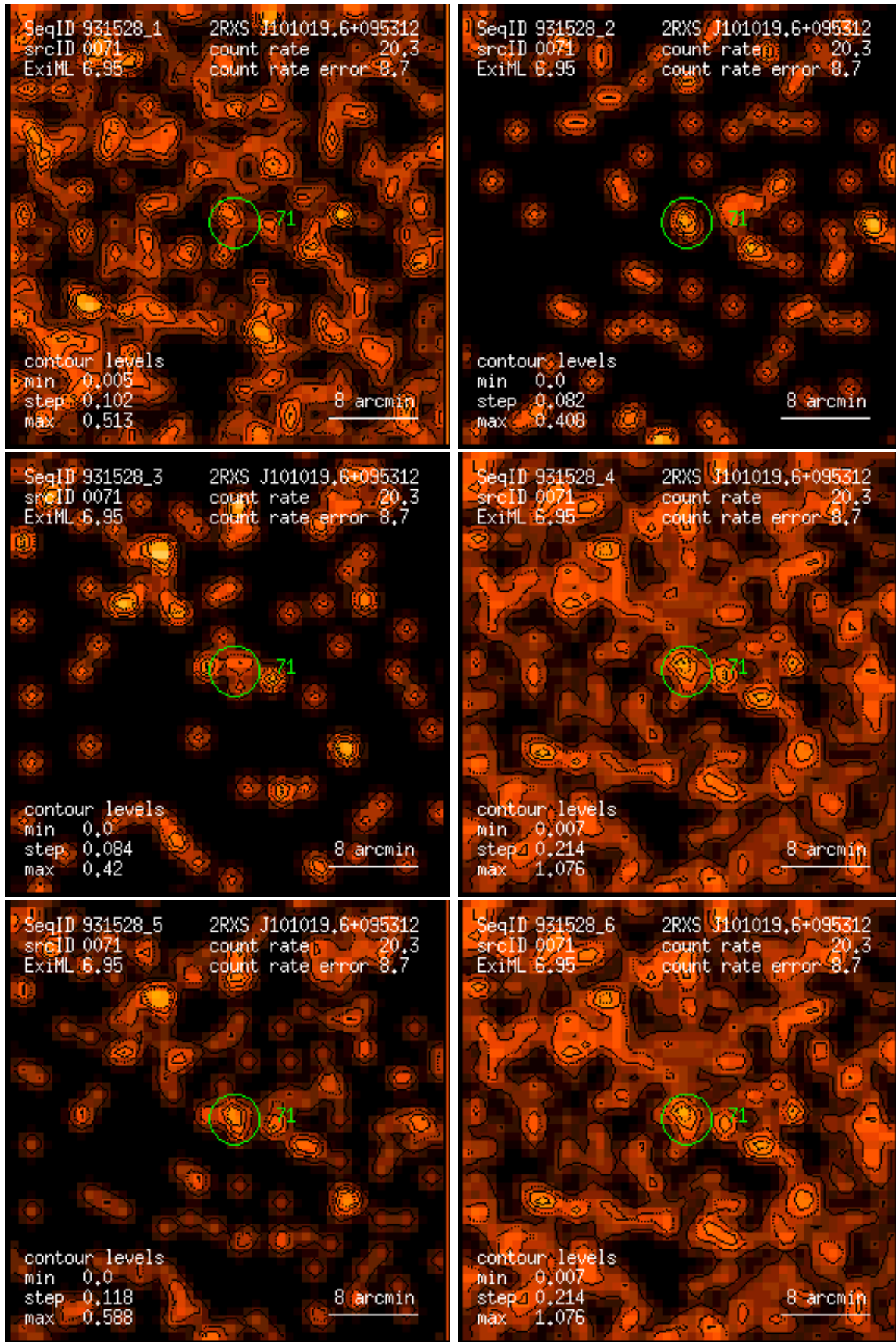
Figure 71: RASS 931528: detection 0071: band rate images, Gaussian filter: (1) PSPC channels 11 – 41, (2) 52 – 90, (3) 91 – 201, (4) 11 – 235, (5) 52 – 201, (6) 11 – 201. Broad band rates in counts/ks. Band rate contour levels in counts/ks/arcmin 2 .
