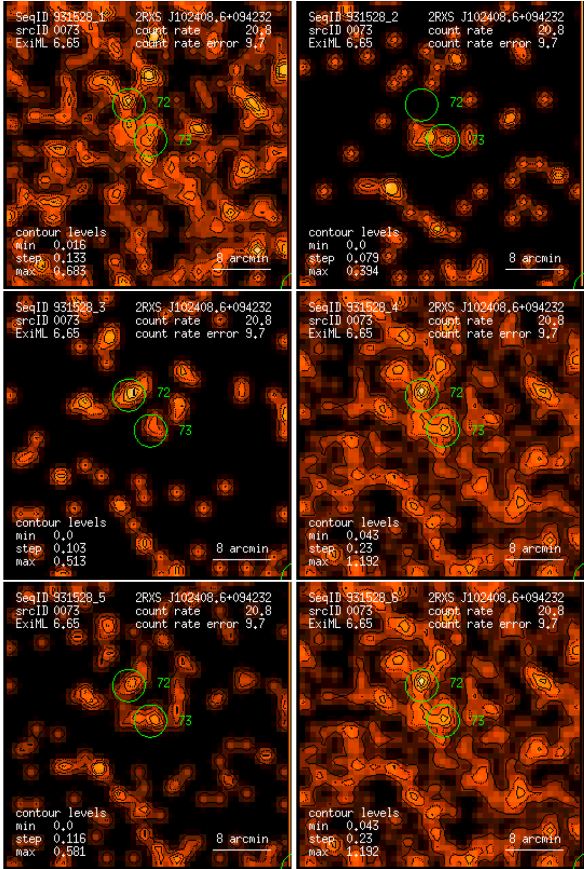
Figure 73: RASS 931528: detection 0073: band rate images, Gaussian filter: (1) PSPC channels 11 – 41, (2) 52 – 90, (3) 91 – 201, (4) 11 – 235, (5) 52 – 201, (6) 11 – 201. Broad band rates in counts/ks. Band rate contour levels in counts/ks/arcmin 2 .
