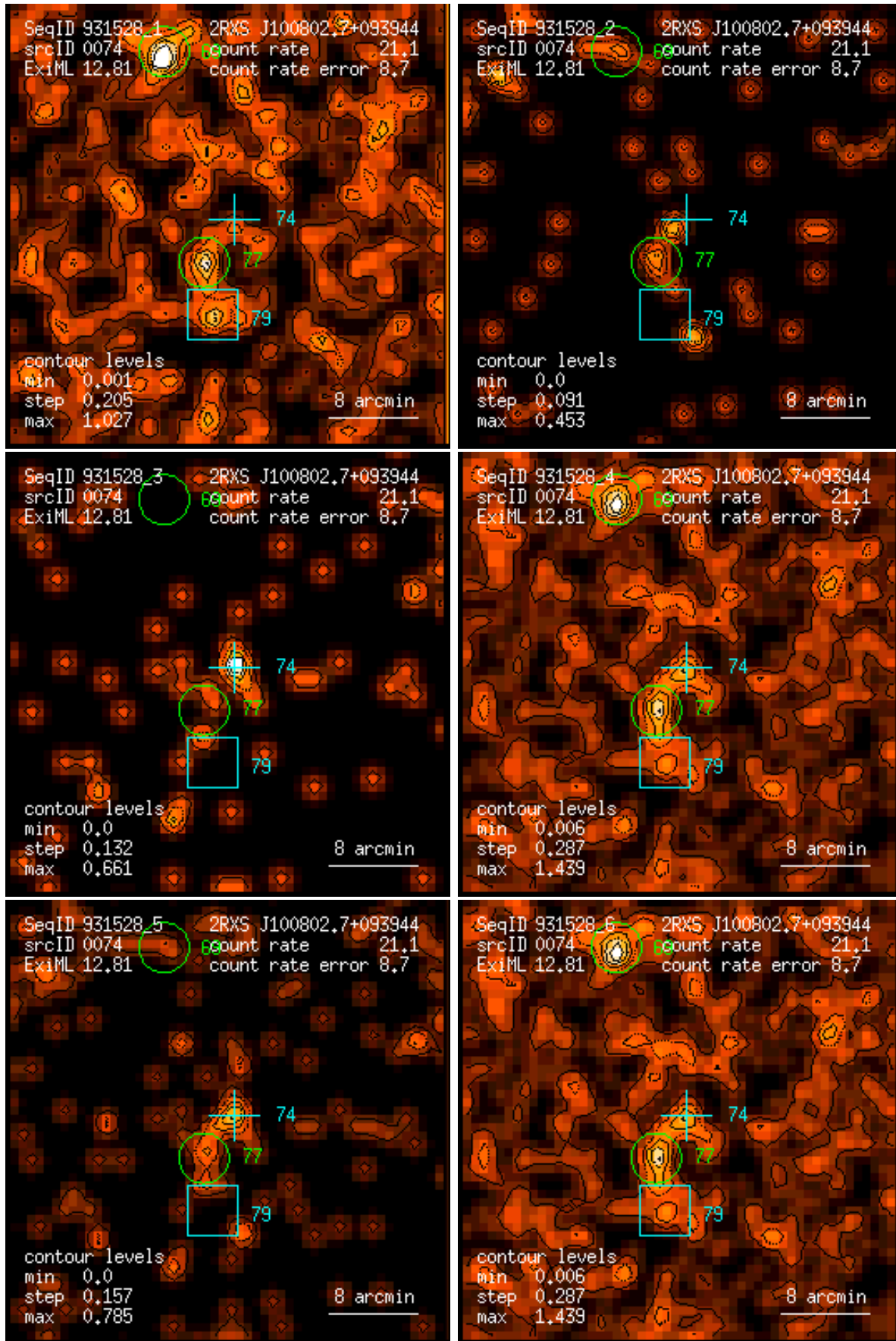
Figure 74: RASS 931528: detection 0074: band rate images, Gaussian filter: (1) PSPC channels 11 – 41, (2) 52 – 90, (3) 91 – 201, (4) 11 – 235, (5) 52 – 201, (6) 11 – 201. Broad band rates in counts/ks. Band rate contour levels in counts/ks/arcmin 2 .
