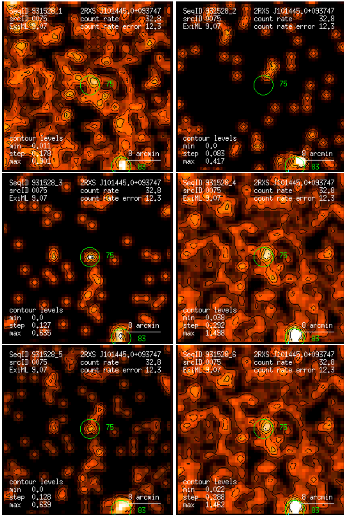
Figure 75: RASS 931528: detection 0075: band rate images, Gaussian filter: (1) PSPC channels 11 – 41, (2) 52 – 90, (3) 91 – 201, (4) 11 – 235, (5) 52 – 201, (6) 11 – 201. Broad band rates in counts/ks. Band rate contour levels in counts/ks/arcmin 2 .
