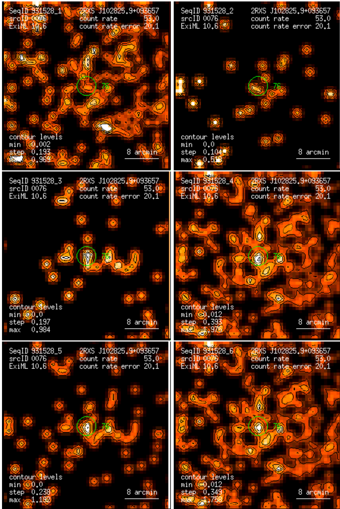
Figure 76: RASS 931528: detection 0076: band rate images, Gaussian filter: (1) PSPC channels 11 – 41, (2) 52 – 90, (3) 91 – 201, (4) 11 – 235, (5) 52 – 201, (6) 11 – 201. Broad band rates in counts/ks. Band rate contour levels in counts/ks/arcmin 2 .
