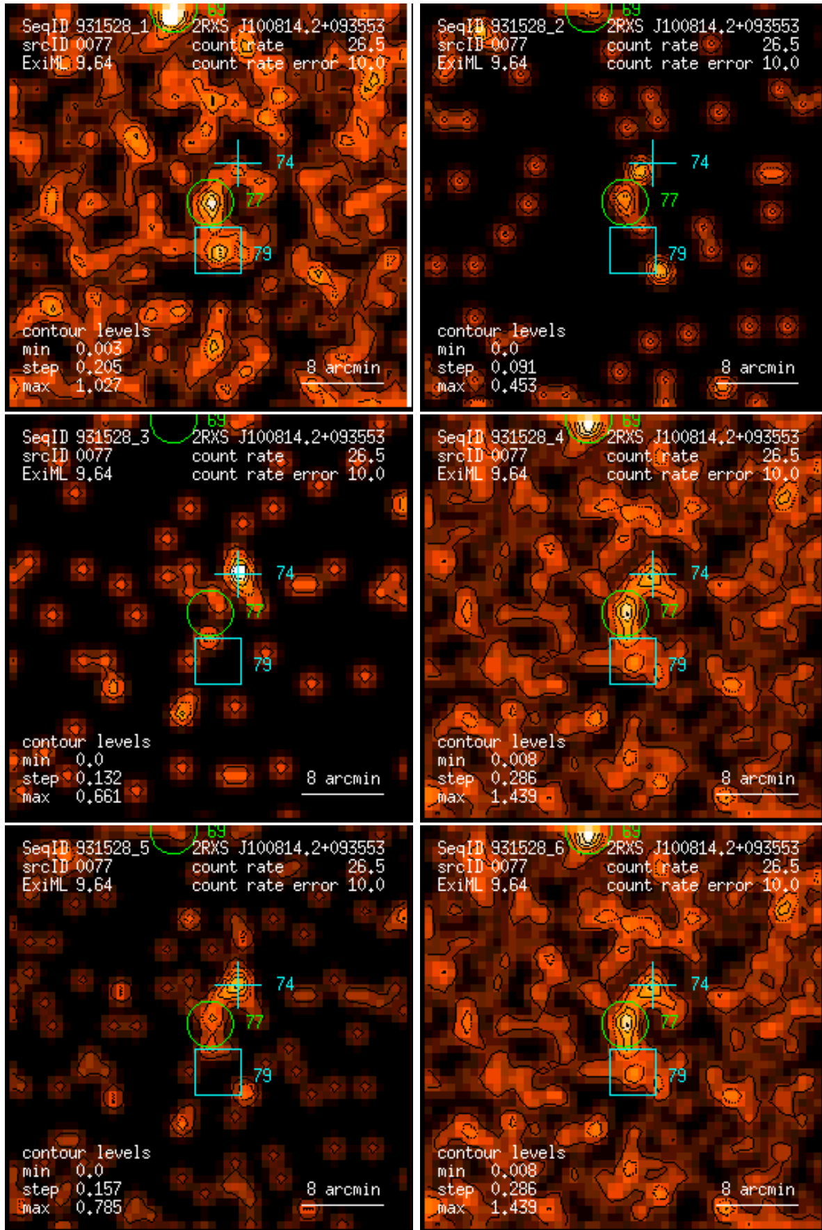
Figure 77: RASS 931528: detection 0077: band rate images, Gaussian filter: (1) PSPC channels 11 – 41, (2) 52 – 90, (3) 91 – 201, (4) 11 – 235, (5) 52 – 201, (6) 11 – 201. Broad band rates in counts/ks. Band rate contour levels in counts/ks/arcmin 2 .
