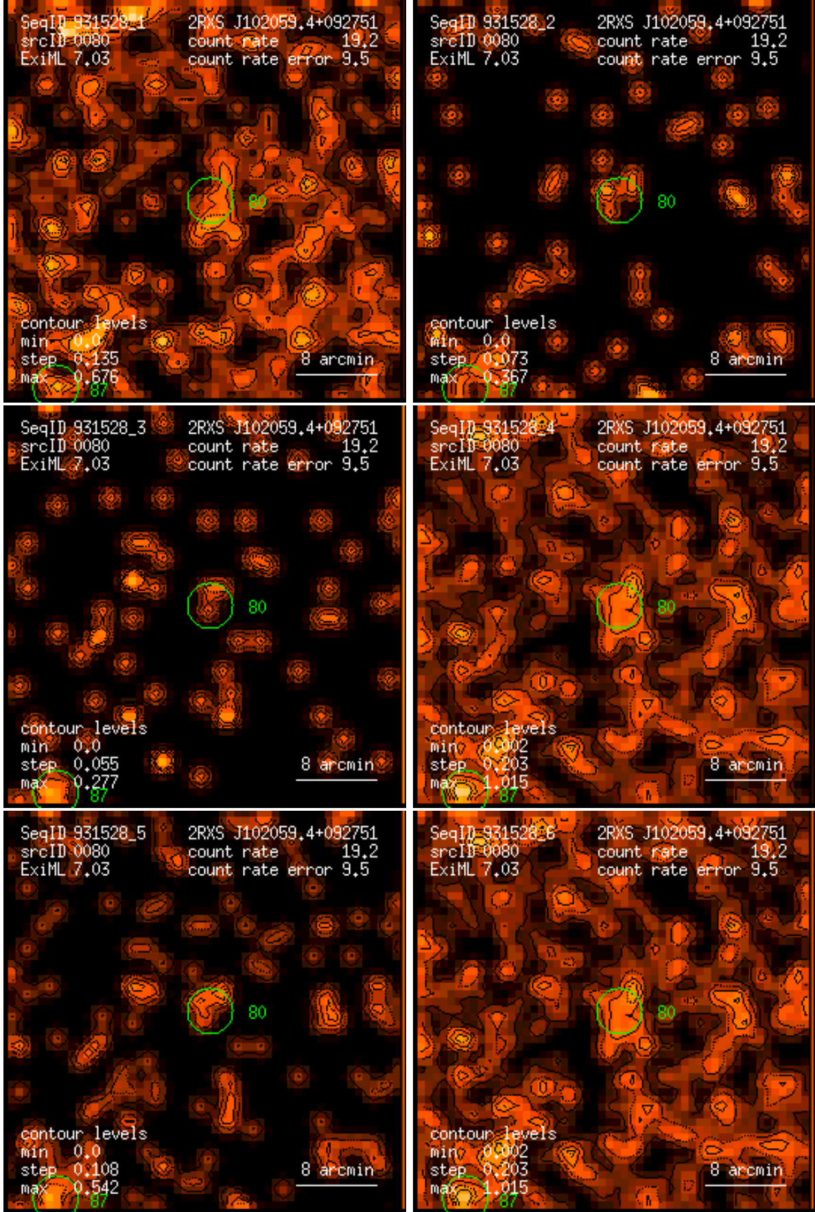
Figure 80: RASS 931528: detection 0080: band rate images, Gaussian filter: (1) PSPC channels 11 – 41, (2) 52 – 90, (3) 91 – 201, (4) 11 – 235, (5) 52 – 201, (6) 11 – 201. Broad band rates in counts/ks. Band rate contour levels in counts/ks/arcmin 2 .
