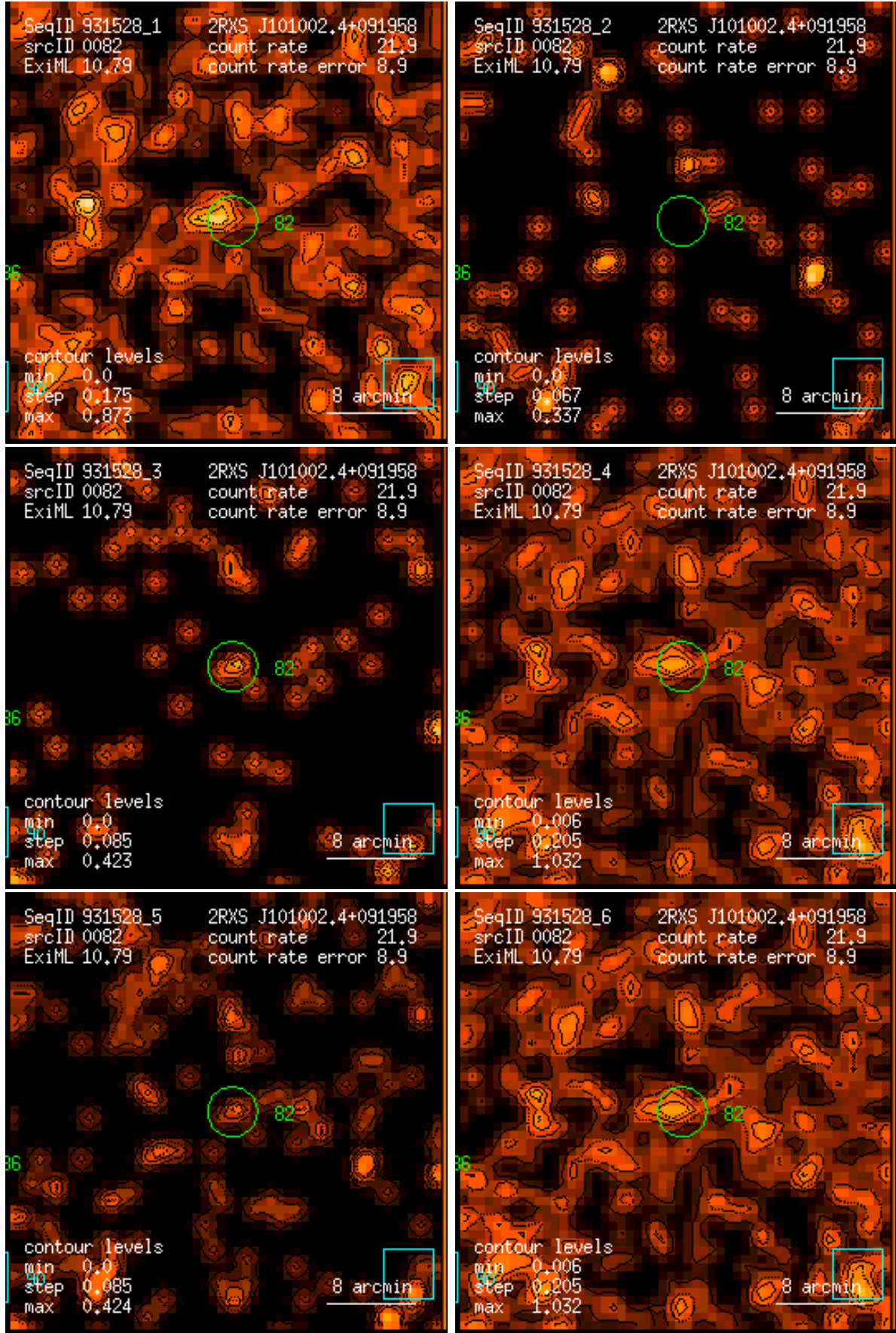
Figure 82: RASS 931528: detection 0082: band rate images, Gaussian filter: (1) PSPC channels 11 – 41, (2) 52 – 90, (3) 91 – 201, (4) 11 – 235, (5) 52 – 201, (6) 11 – 201. Broad band rates in counts/ks. Band rate contour levels in counts/ks/arcmin 2 .
