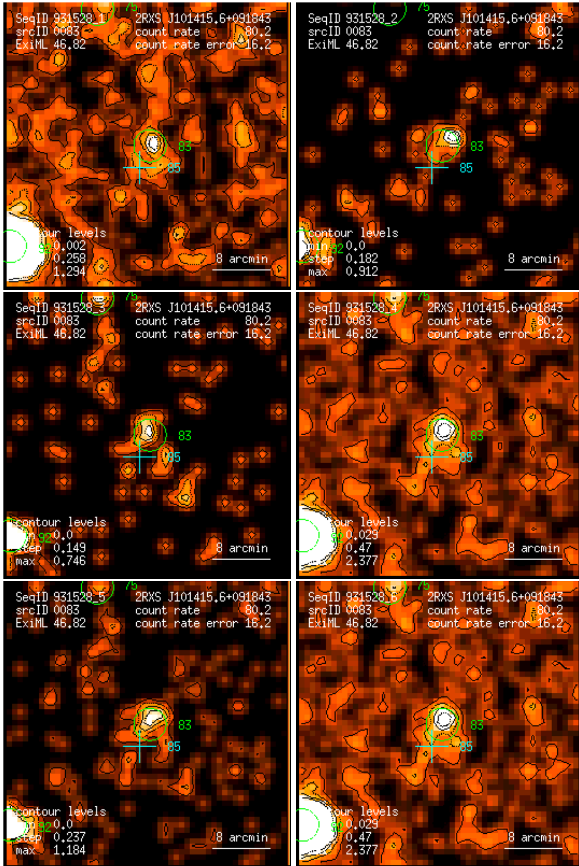
Figure 83: RASS 931528: detection 0083: band rate images, Gaussian filter: (1) PSPC channels 11 – 41, (2) 52 – 90, (3) 91 – 201, (4) 11 – 235, (5) 52 – 201, (6) 11 – 201. Broad band rates in counts/ks. Band rate contour levels in counts/ks/arcmin 2 .
