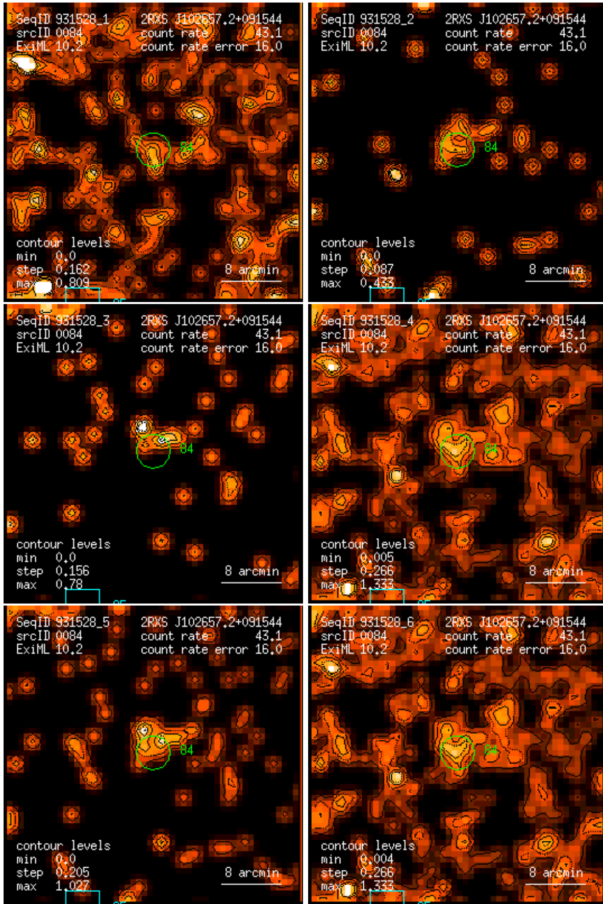
Figure 84: RASS 931528: detection 0084: band rate images, Gaussian filter: (1) PSPC channels 11 – 41, (2) 52 – 90, (3) 91 – 201, (4) 11 – 235, (5) 52 – 201, (6) 11 – 201. Broad band rates in counts/ks. Band rate contour levels in counts/ks/arcmin 2 .
