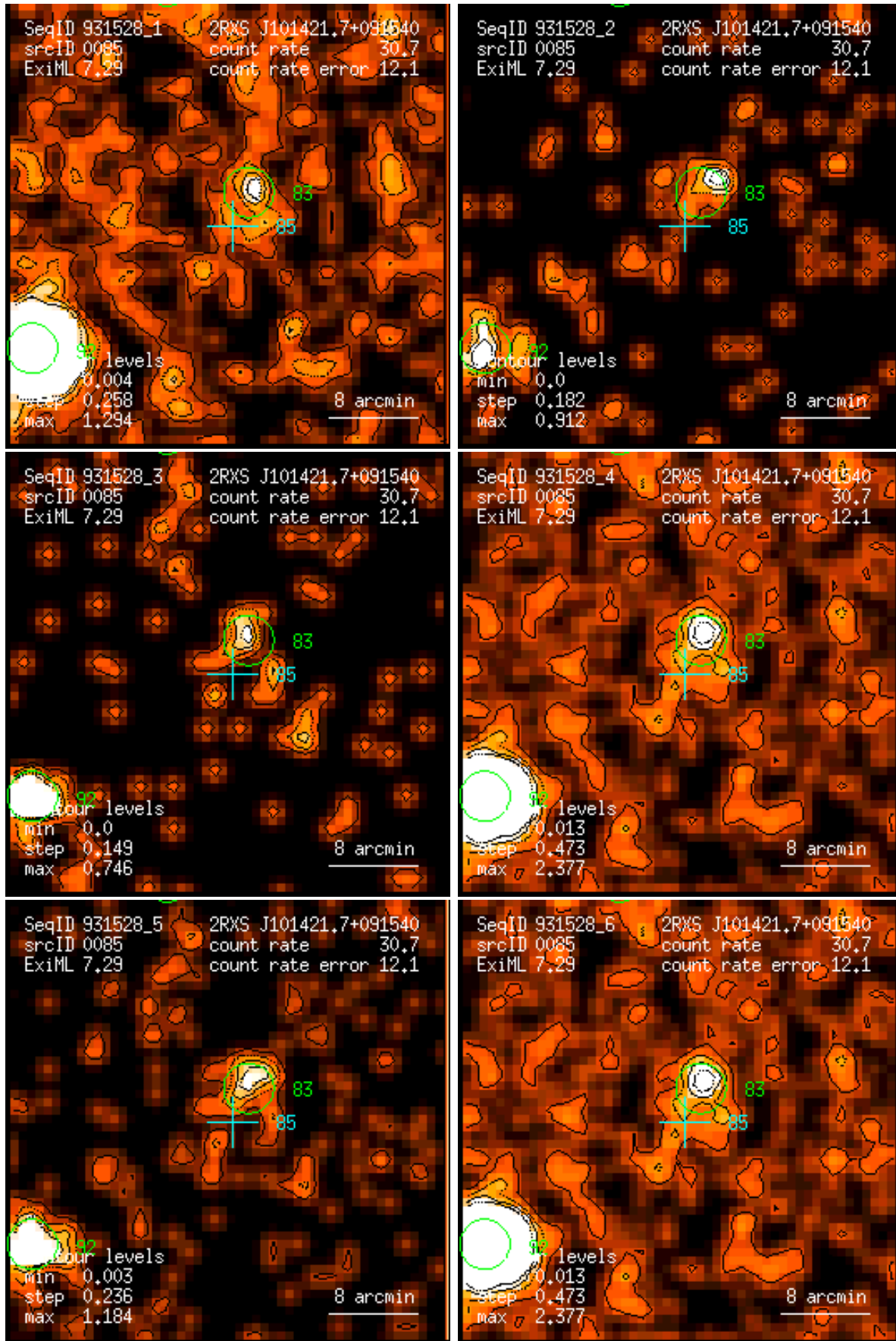
Figure 85: RASS 931528: detection 0085: band rate images, Gaussian filter: (1) PSPC channels 11 – 41, (2) 52 – 90, (3) 91 – 201, (4) 11 – 235, (5) 52 – 201, (6) 11 – 201. Broad band rates in counts/ks. Band rate contour levels in counts/ks/arcmin 2 .
