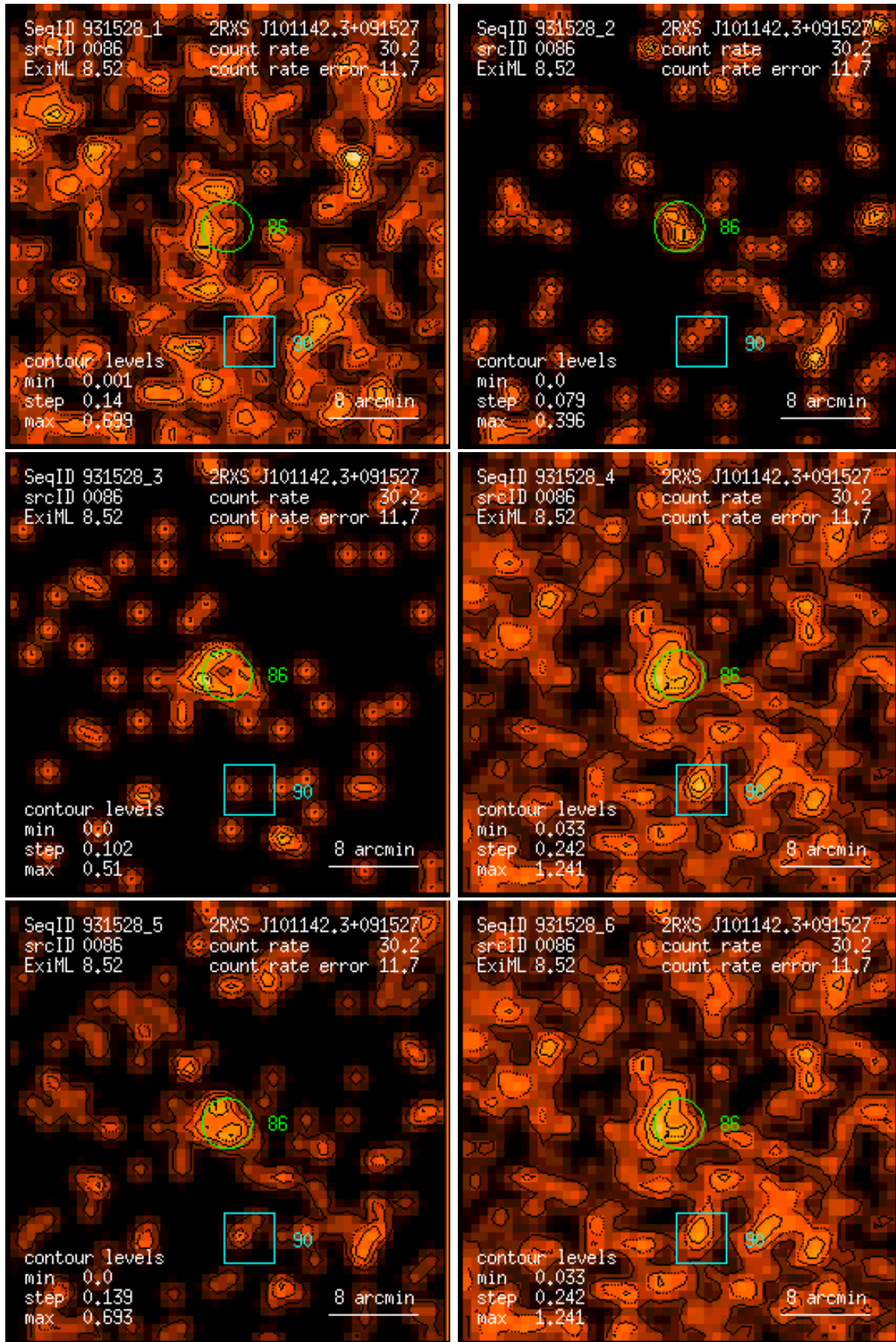
Figure 86: RASS 931528: detection 0086: band rate images, Gaussian filter: (1) PSPC channels 11 – 41, (2) 52 – 90, (3) 91 – 201, (4) 11 – 235, (5) 52 – 201, (6) 11 – 201. Broad band rates in counts/ks. Band rate contour levels in counts/ks/arcmin 2 .
