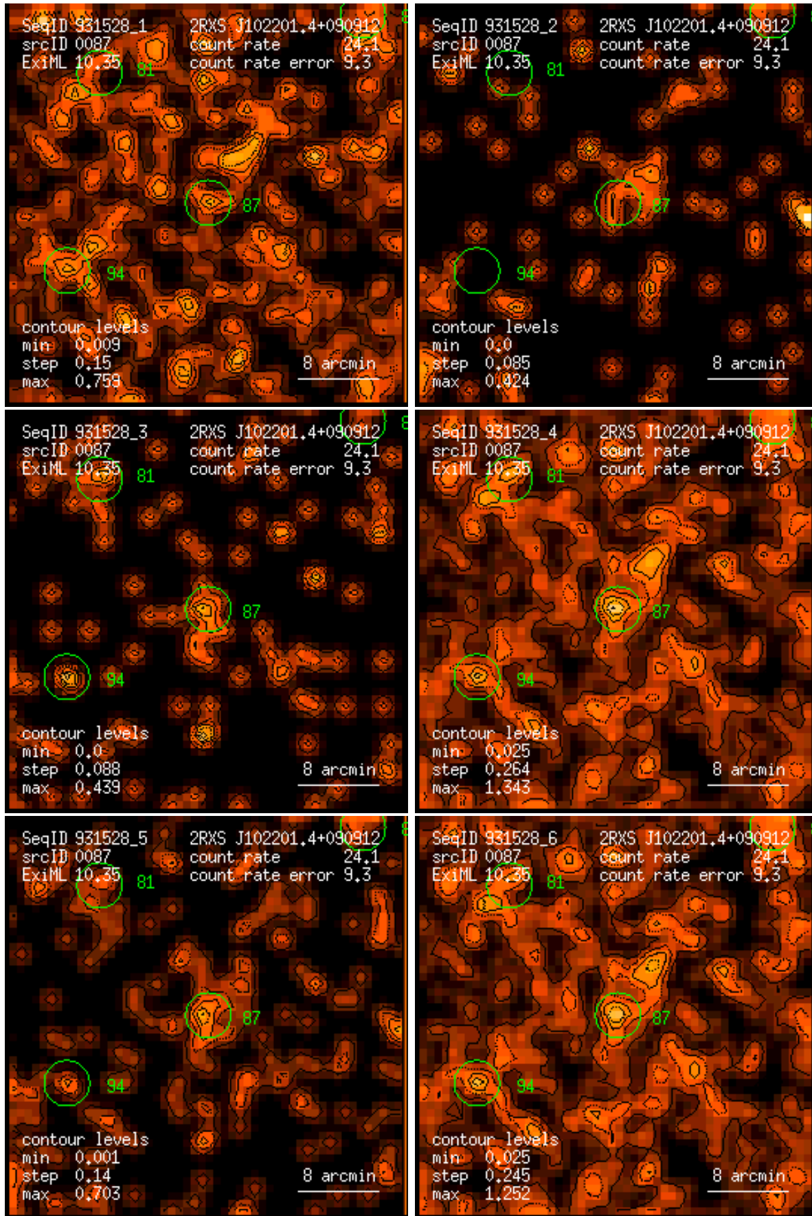
Figure 87: RASS 931528: detection 0087: band rate images, Gaussian filter: (1) PSPC channels 11 – 41, (2) 52 – 90, (3) 91 – 201, (4) 11 – 235, (5) 52 – 201, (6) 11 – 201. Broad band rates in counts/ks. Band rate contour levels in counts/ks/arcmin 2 .
