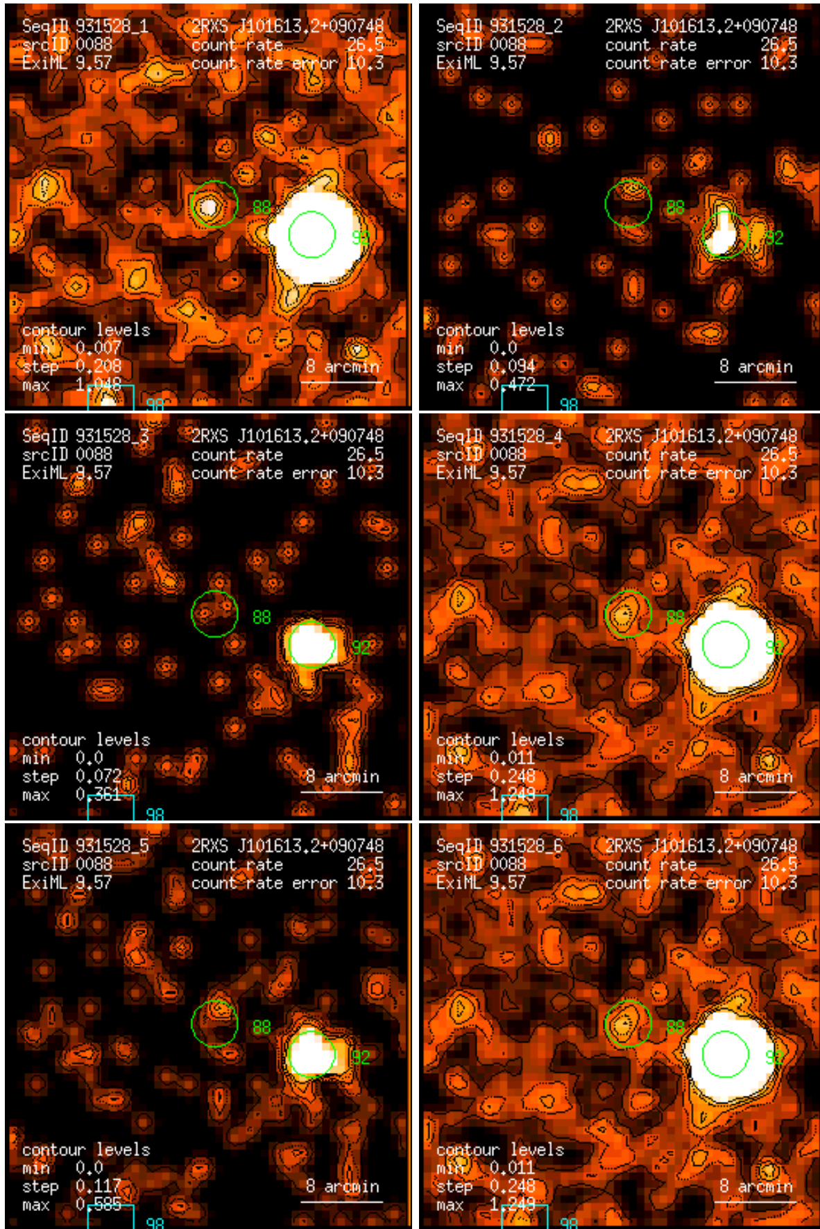
Figure 88: RASS 931528: detection 0088: band rate images, Gaussian filter: (1) PSPC channels 11 – 41, (2) 52 – 90, (3) 91 – 201, (4) 11 – 235, (5) 52 – 201, (6) 11 – 201. Broad band rates in counts/ks. Band rate contour levels in counts/ks/arcmin 2 .
