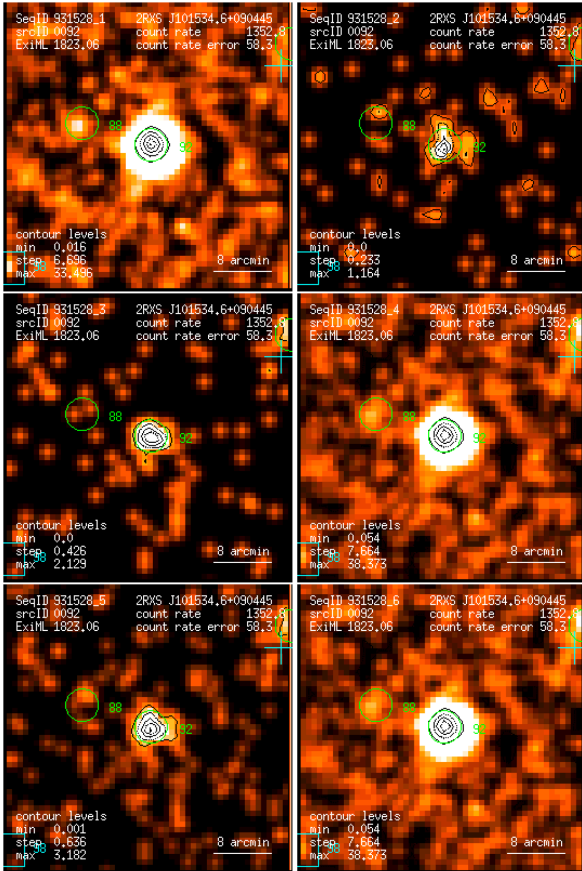
Figure 92: RASS 931528: detection 0092: band rate images, Gaussian filter: (1) PSPC channels 11 – 41, (2) 52 – 90, (3) 91 – 201, (4) 11 – 235, (5) 52 – 201, (6) 11 – 201. Broad band rates in counts/ks. Band rate contour levels in counts/ks/arcmin 2 .
