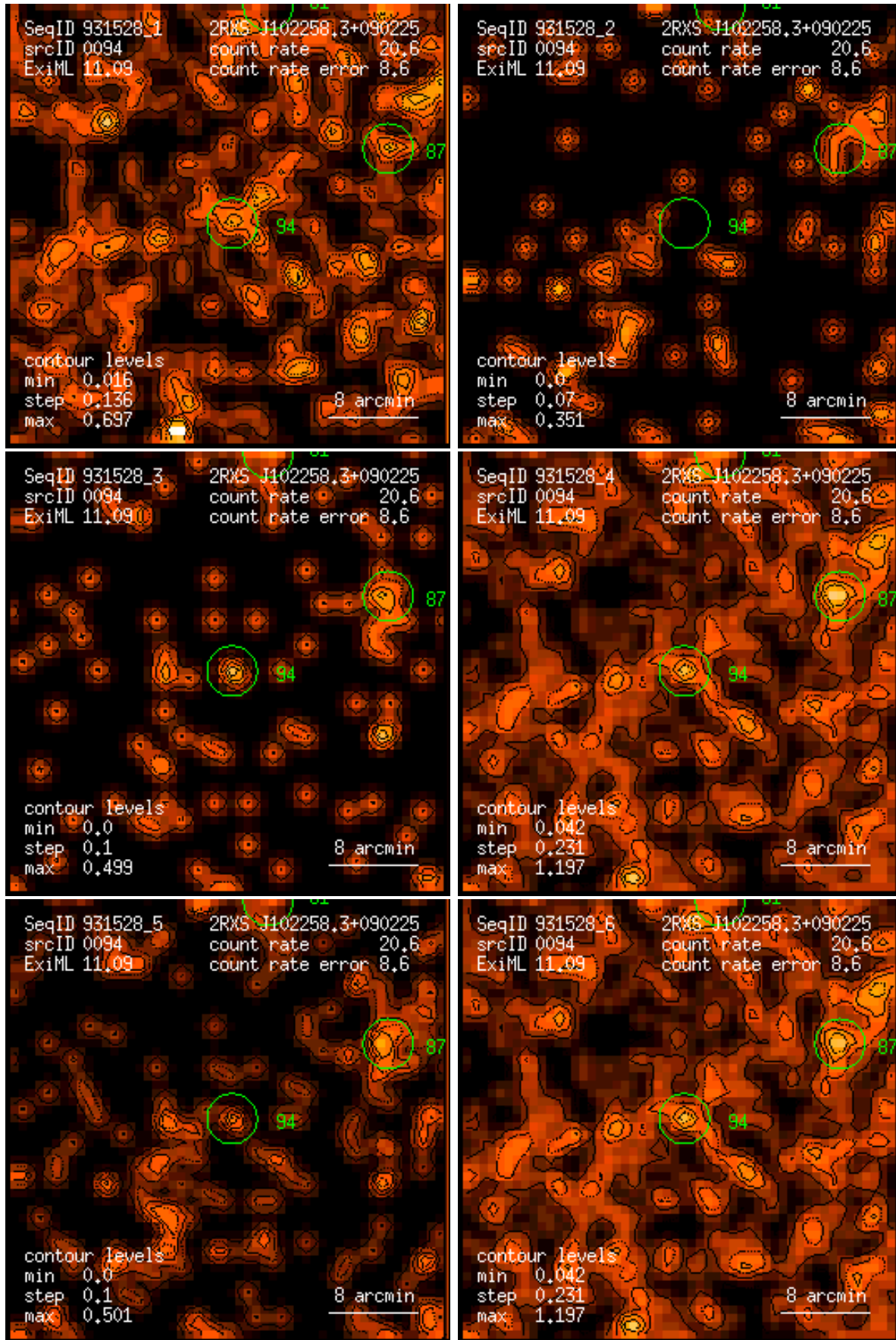
Figure 94: RASS 931528: detection 0094: band rate images, Gaussian filter: (1) PSPC channels 11 – 41, (2) 52 – 90, (3) 91 – 201, (4) 11 – 235, (5) 52 – 201, (6) 11 – 201. Broad band rates in counts/ks. Band rate contour levels in counts/ks/arcmin 2 .
